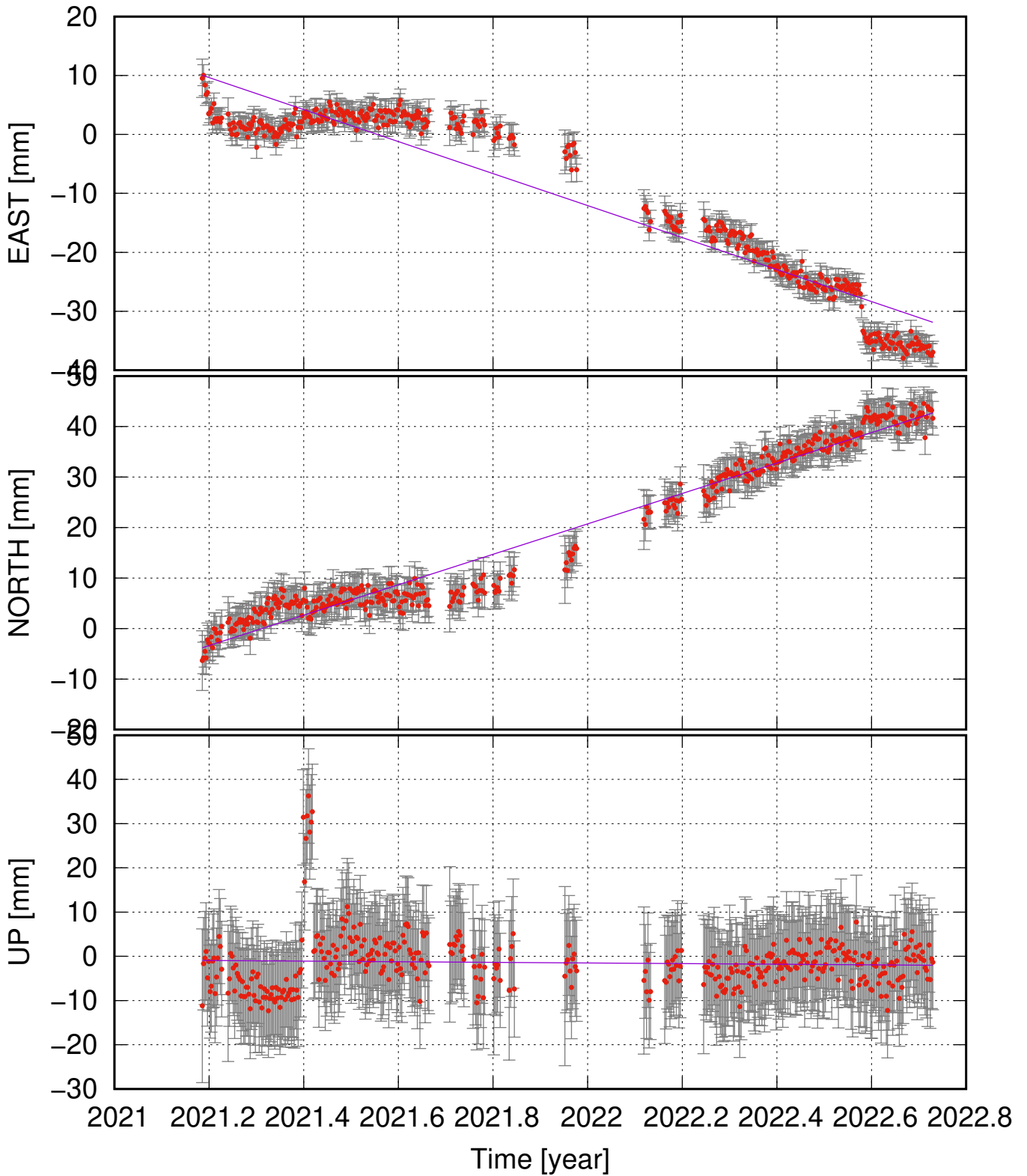
HAFC (63.93, -22.68) time series (ITRF 2014) v_e = -27.15 \pm 2.88 ; v_n = 30.11 \pm 1.88 ; v_u = -0.69 \pm 4.00 mm/yr
