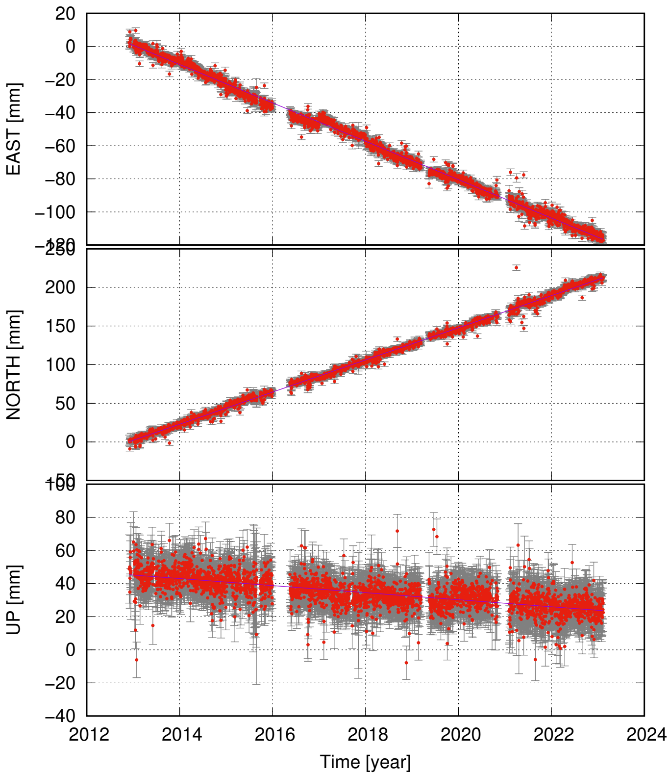
GUSK (64.89, -23.92) time series (ITRF 2014) ve = -11.60 \pm 0.23 ; vn = 20.82 \pm 0.31 ; vu = -2.13 \pm 0.65 mm/yr
