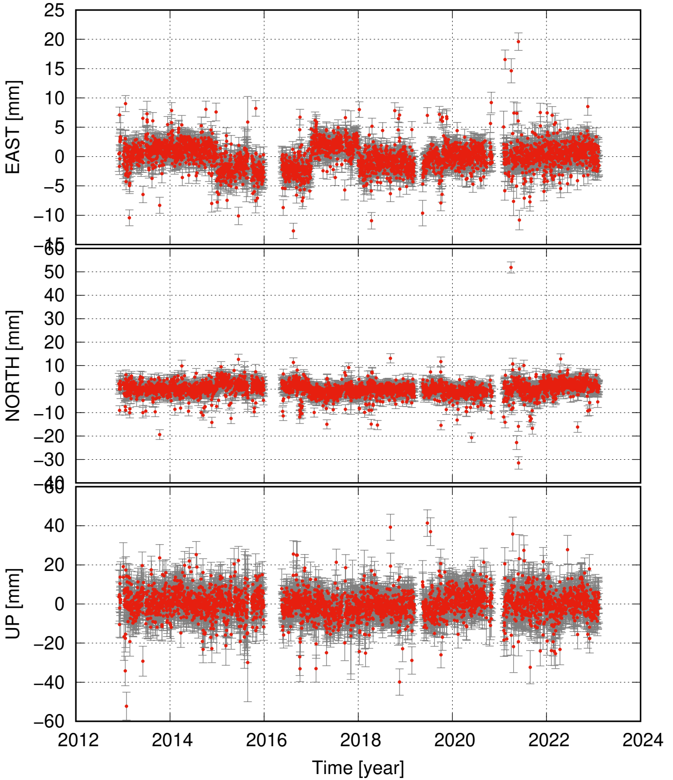
GUSK detrended and seasonal signal removed
