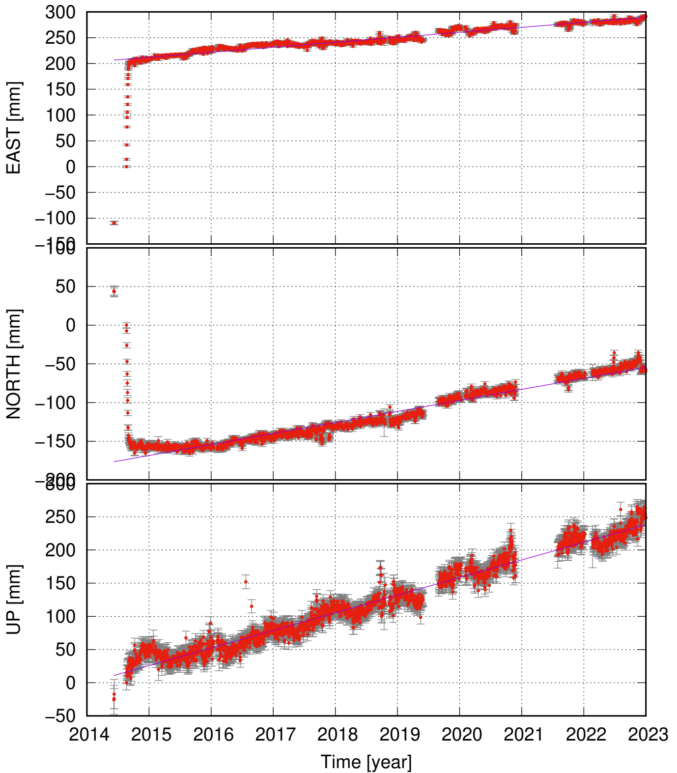
GSIG (64.68, -16.68) time series (ITRF 2014) v_e = 9.67 \pm 1.68 ; v_n = 14.23 \pm 1.47 ; v_u = 26.52 \pm 1.39 mm/yr
