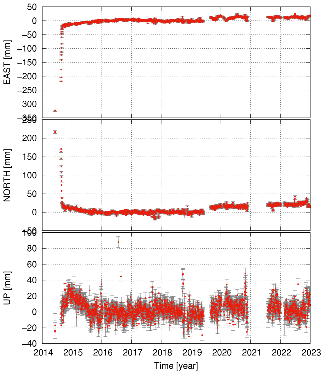
GSIG detrended and seasonal signal removed
