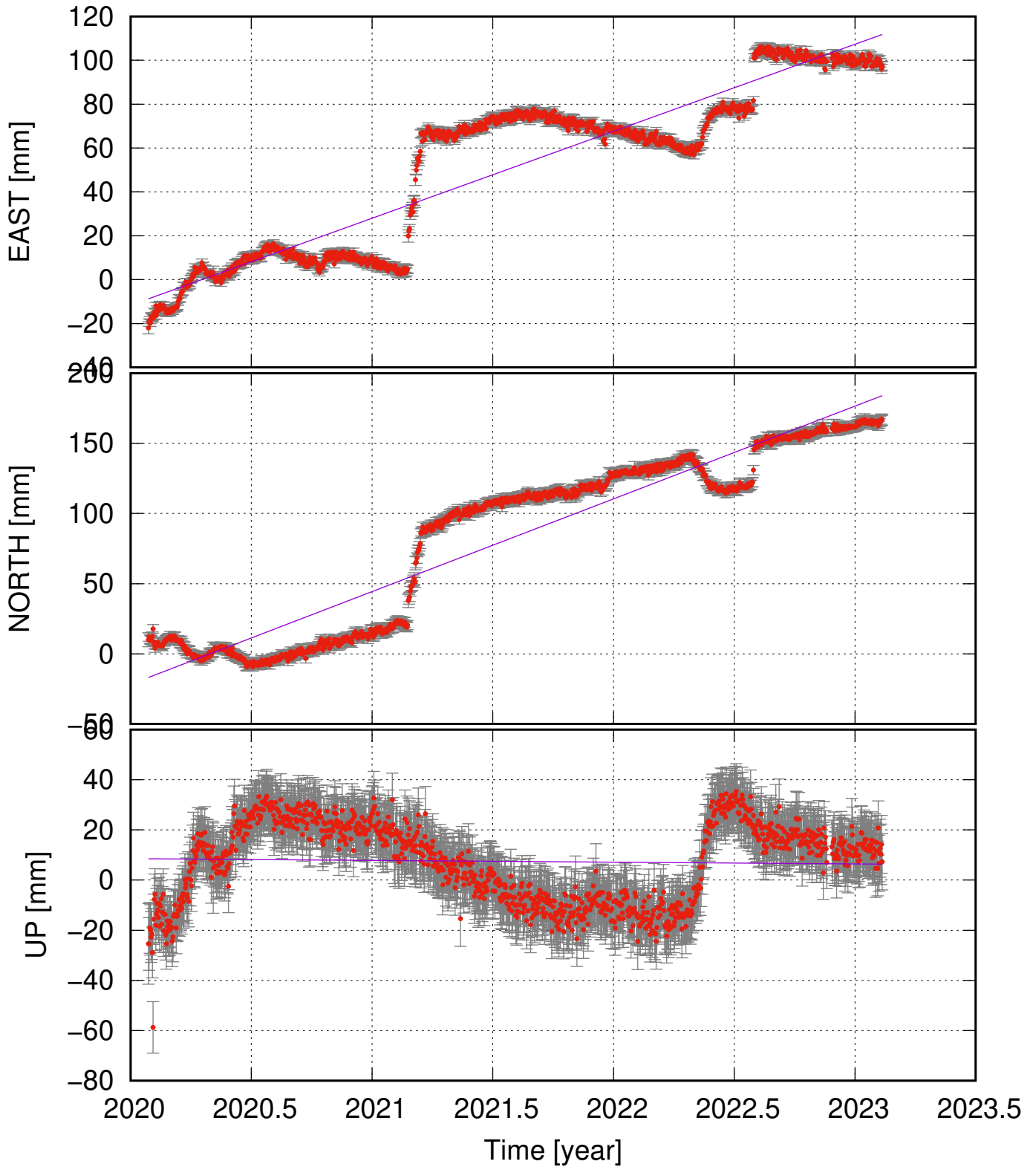
GRIC (63.85, -22.43) time series (ITRF 2014) v_e = 39.64 \pm 4.79 ; v_n = 66.03 \pm 6.71 ; v_u = -0.71 \pm 5.17 mm/yr
