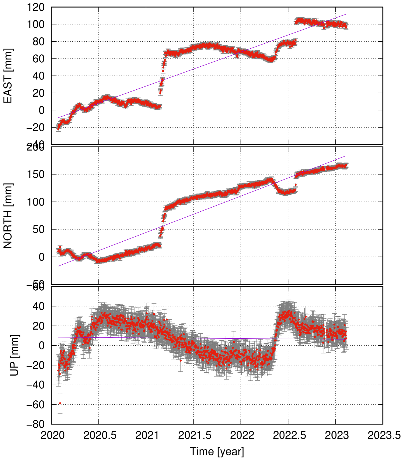
GRIC (63.85, -22.43) time series (ITRF 2014) ve = 39.64 ± 4.79; vn = 66.03 ± 6.71; vu = -0.71 ± 5.17 mm/yr
