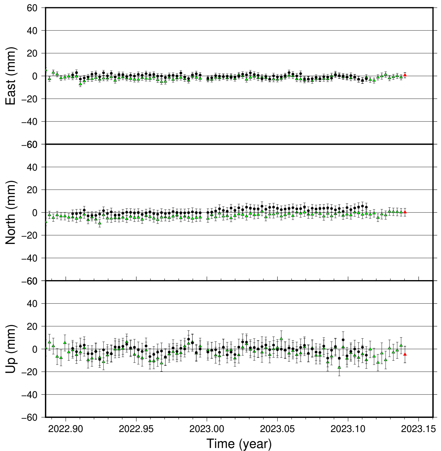
GRIC time series (IGS 2014), last 100 days
