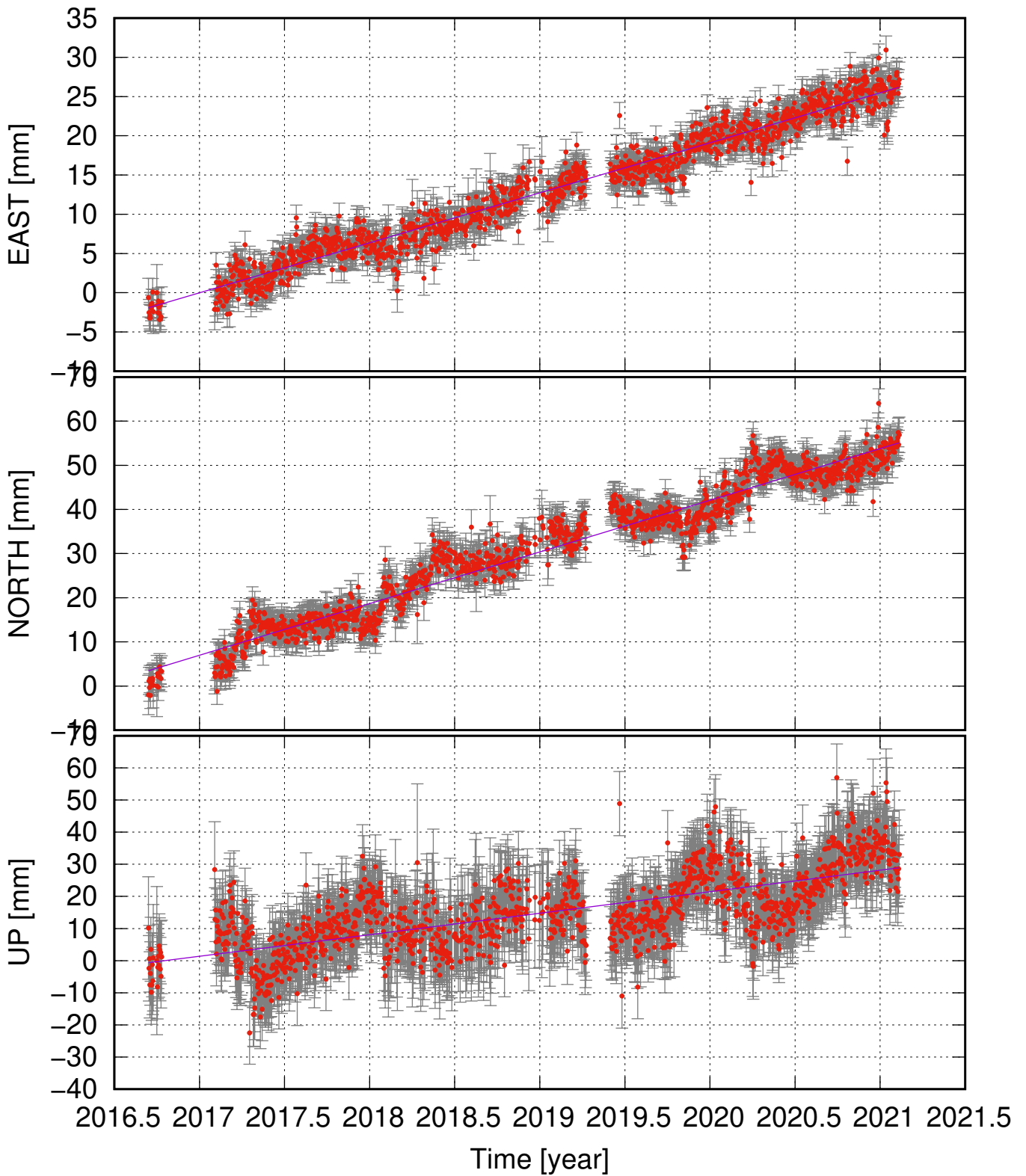
GRFS (63.53, -19.11) time series (ITRF 2014) v_e = 6.37 \pm 0.38 ; v_n = 11.71 \pm 0.77 ; v_u = 6.70 \pm 1.88 mm/yr
