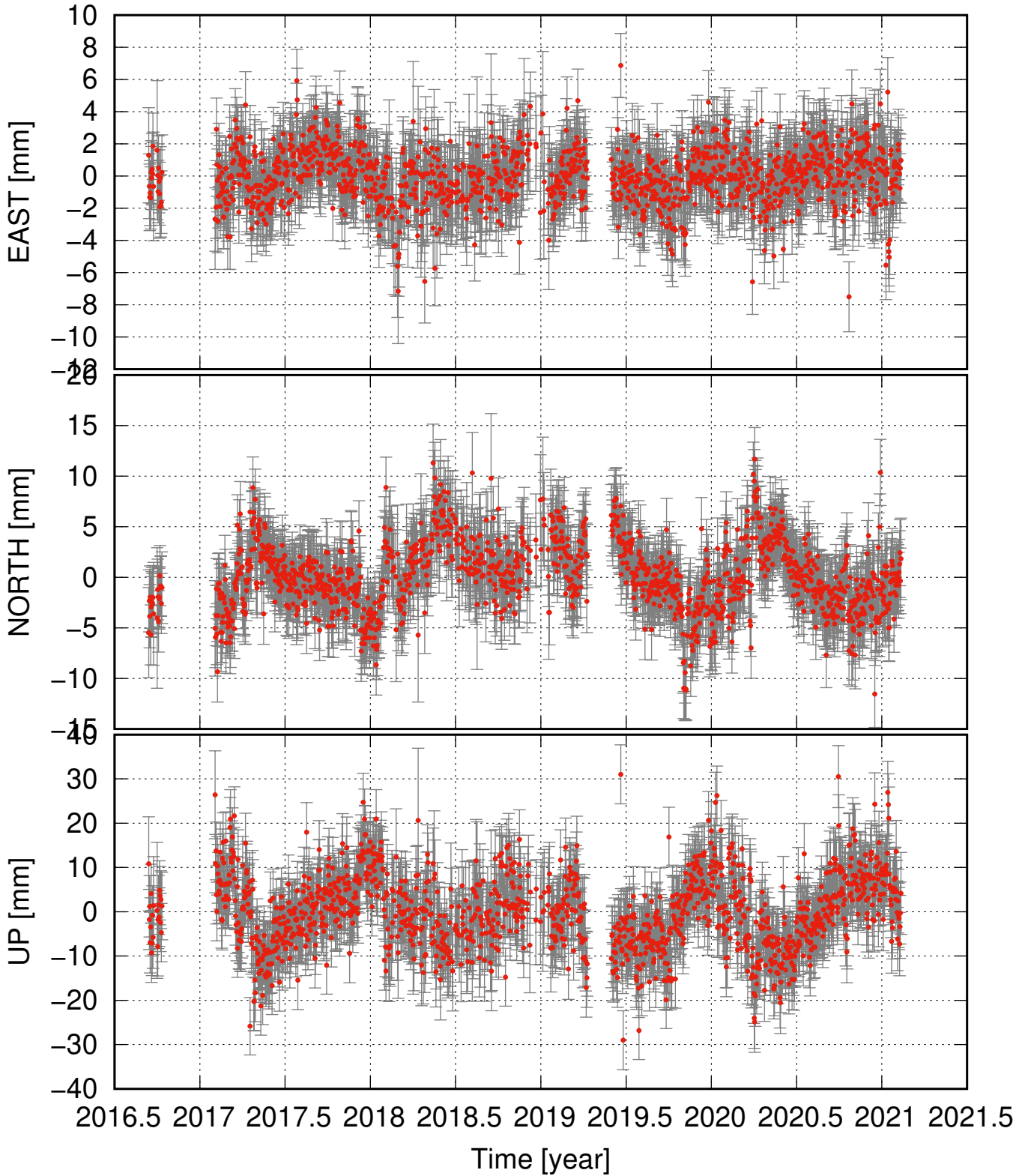
GRFS residual time series (some major events removed as well)
