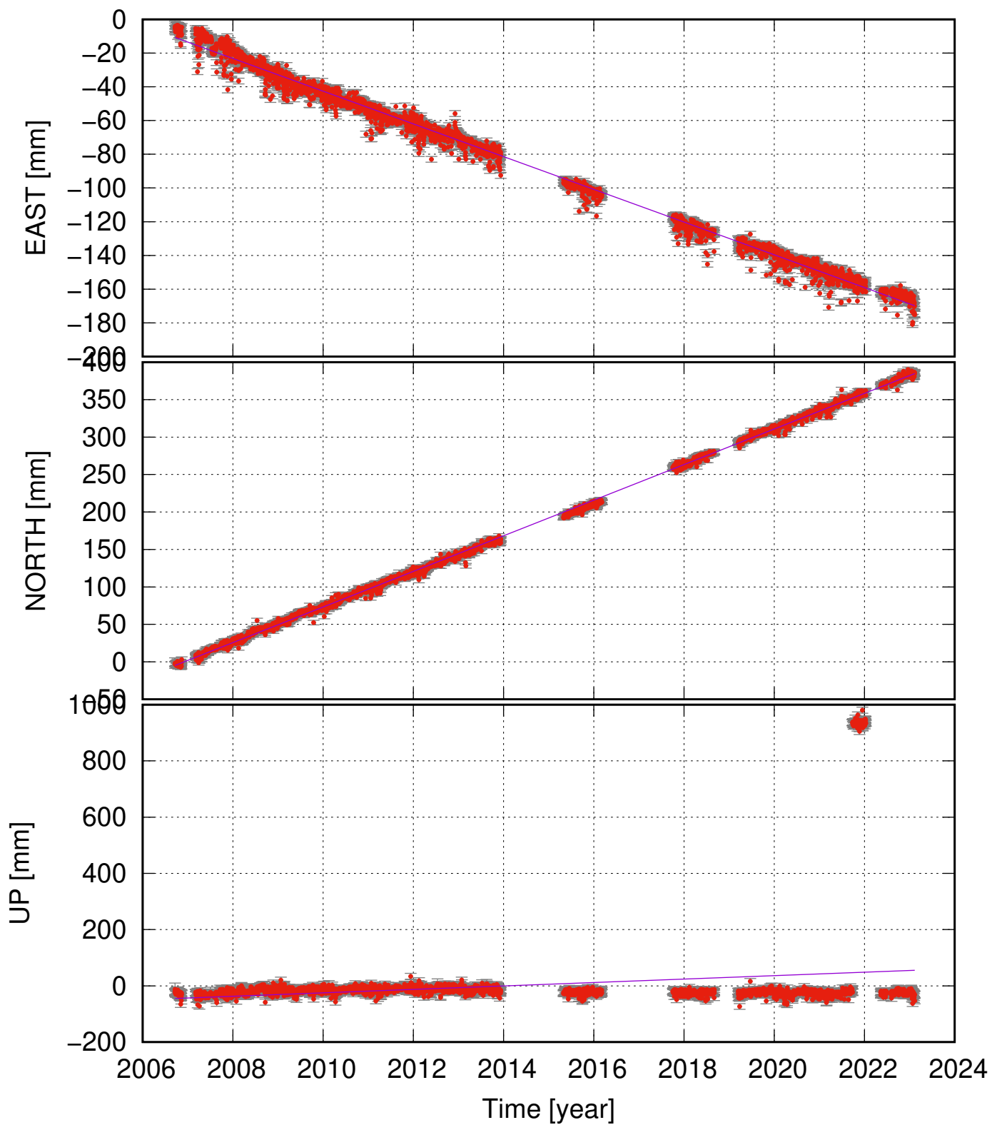
GRAN (65.92, -17.58) time series (ITRF 2014) v_e = -9.71 \pm 0.21 ; v_n = 23.75 \pm 0.19 ; v_u = 6.11 \pm 8.91 mm/yr
