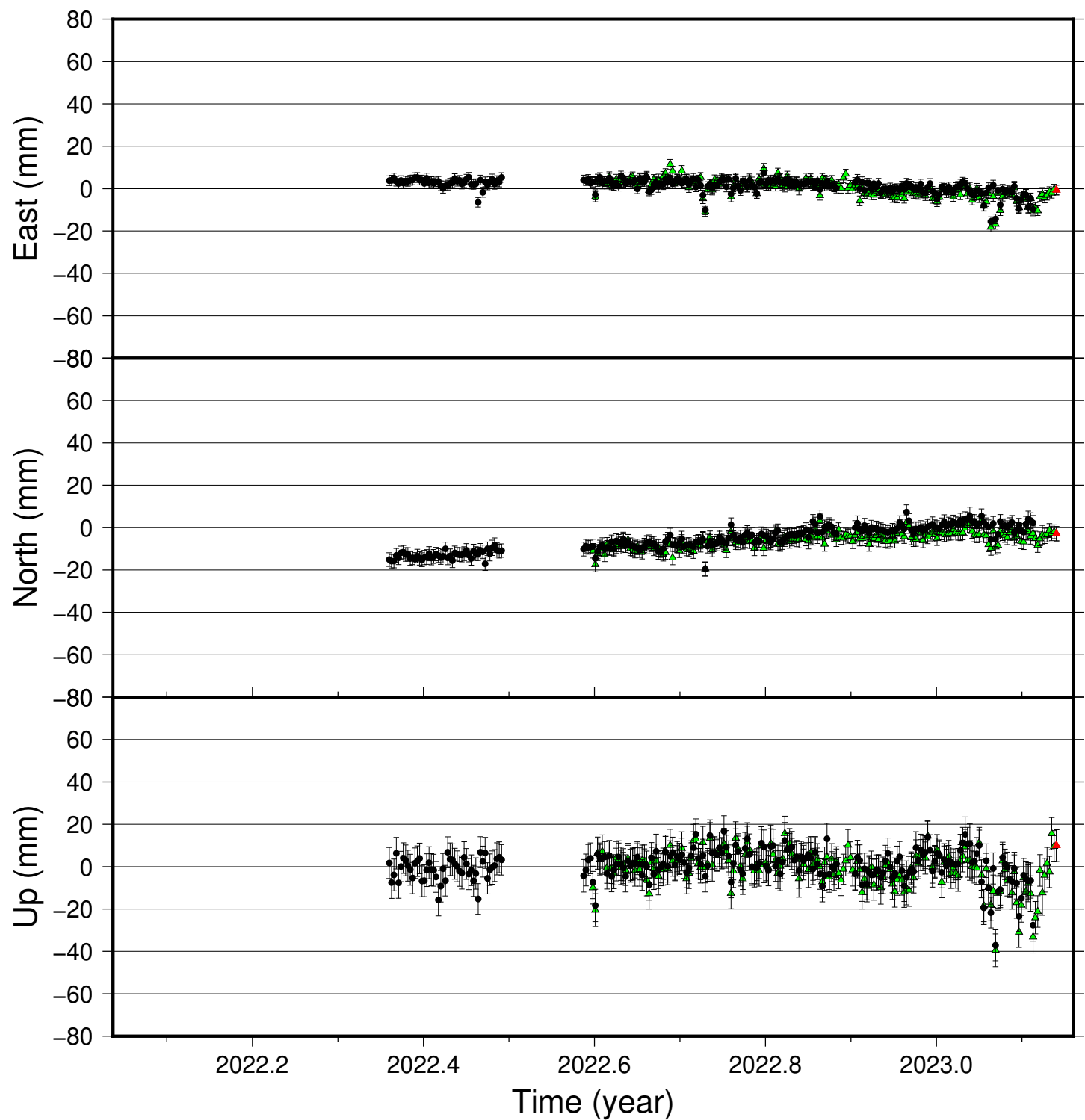
GRAN time series (IGS 2014), last 400 days
