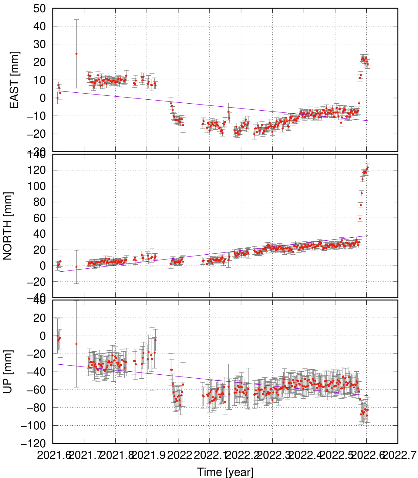
GONH (63.89, -22.27) time series (ITRF 2014) ve = -16.86 ± 10.13; vn = 46.15 ± 15.50; vu = -35.45 ± 12.50 mm/yr
