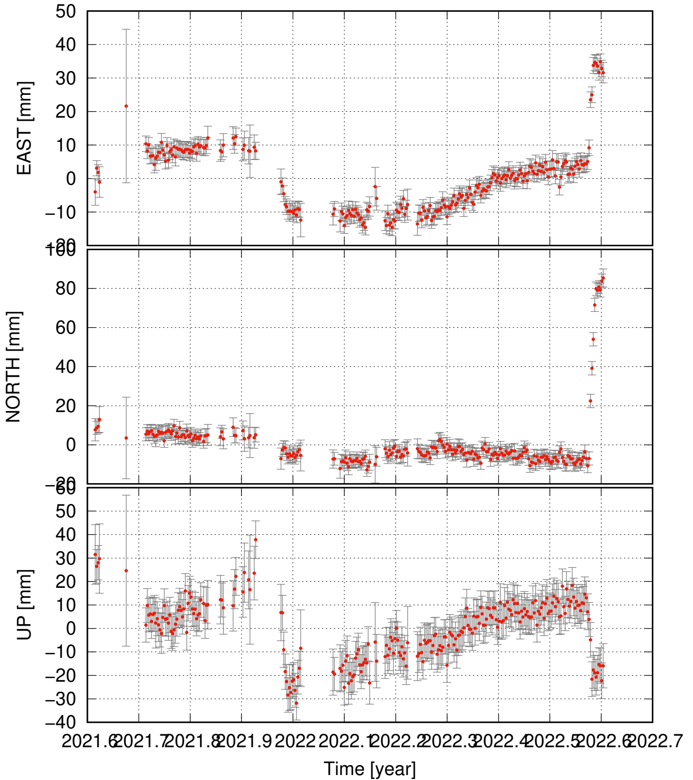
GONH residual time series (some major events removed as well)
