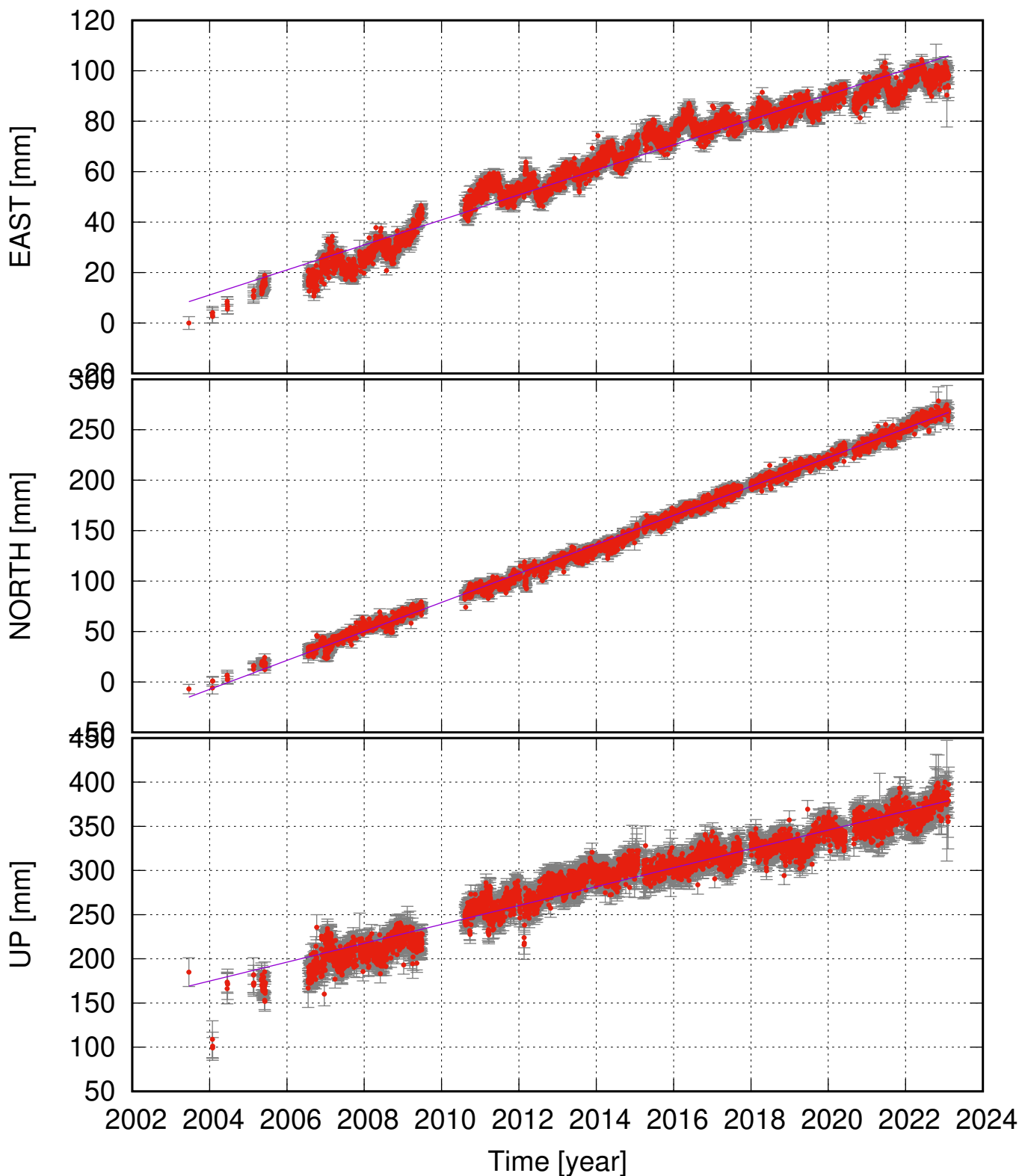
GOLA (63.66, -19.32) time series (ITRF 2014) v_e = 4.96 \pm 0.25 ; v_n = 14.37 \pm 0.20 ; v_u = 10.68 \pm 0.61 mm/yr
