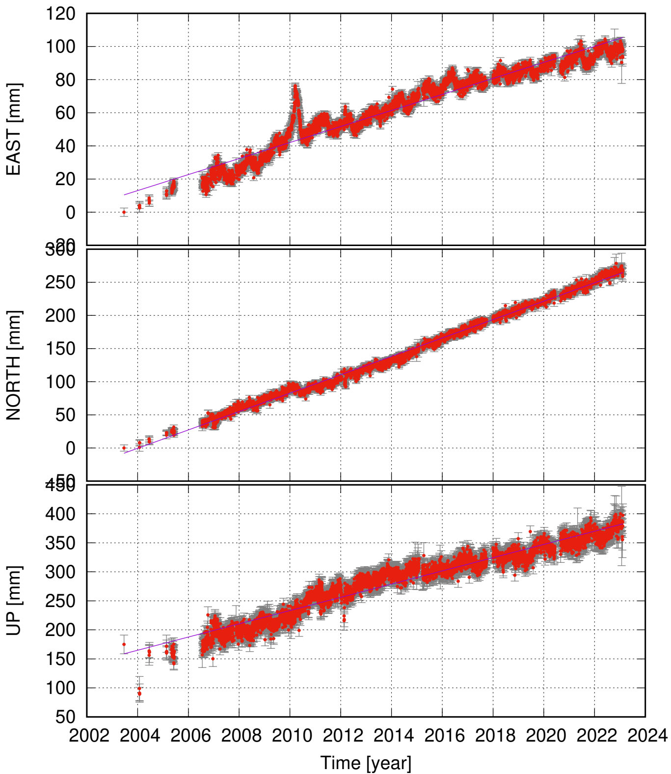
GOLA (63.66, -19.32) time series (ITRF 2014) v_e = 4.84 \pm 0.29 ; v_n = 13.87 \pm 0.26 ; v_u = 11.40 \pm 0.68 mm/yr
