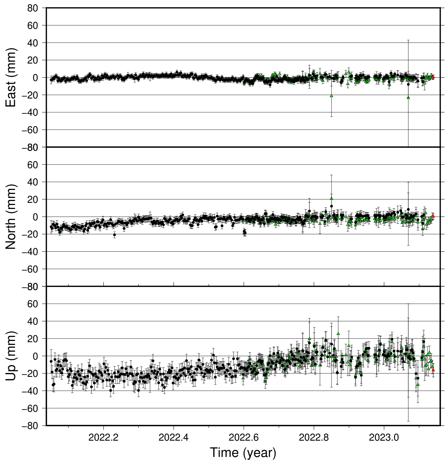
GOLA time series (IGS 2014), last 400 days
