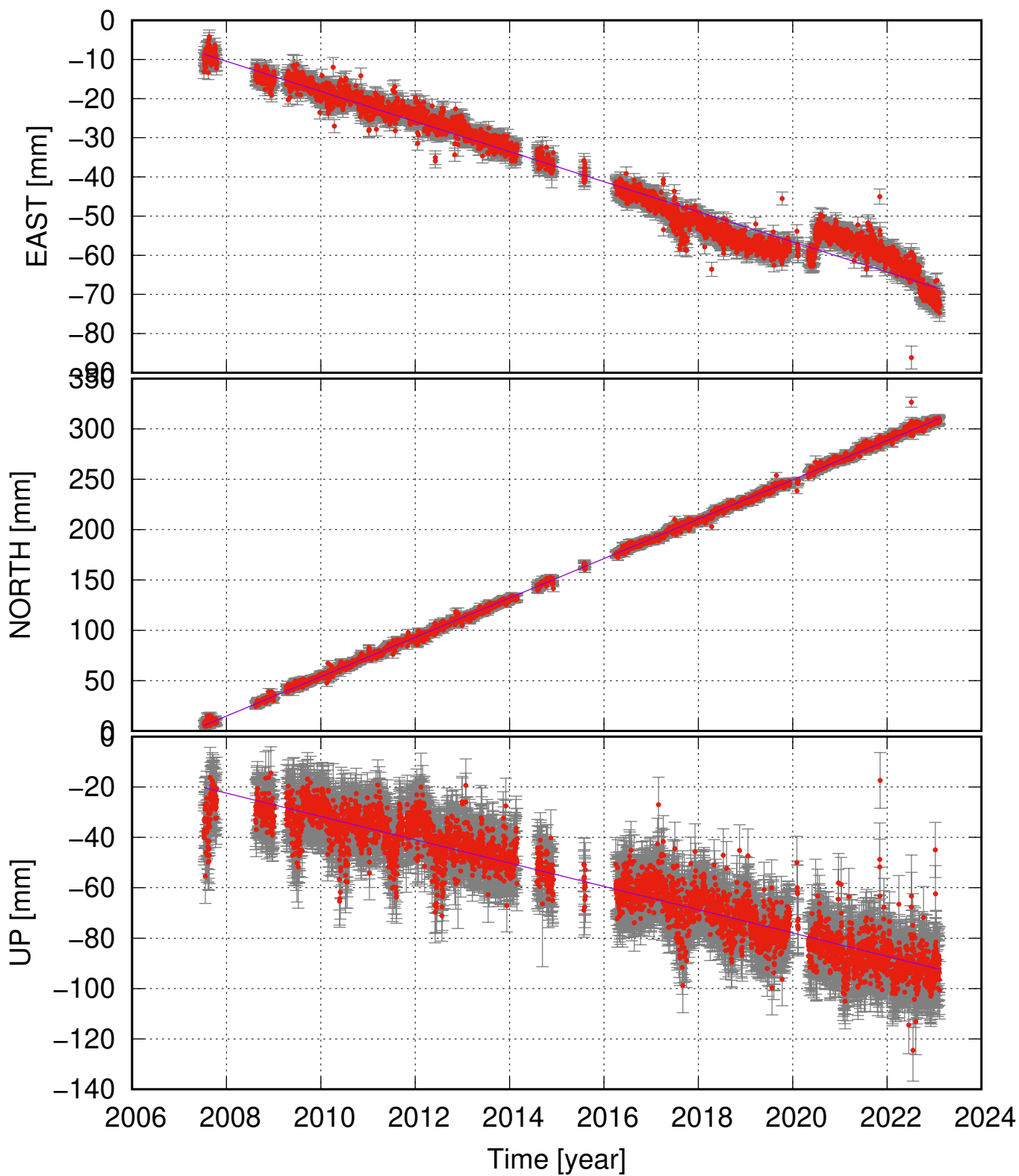
GMEY (66.54, -18.02) time series (ITRF 2014) v_e = -3.84 \pm 0.20 ; v_n = 19.55 \pm 0.13 ; v_u = -4.63 \pm 0.44 mm/yr
