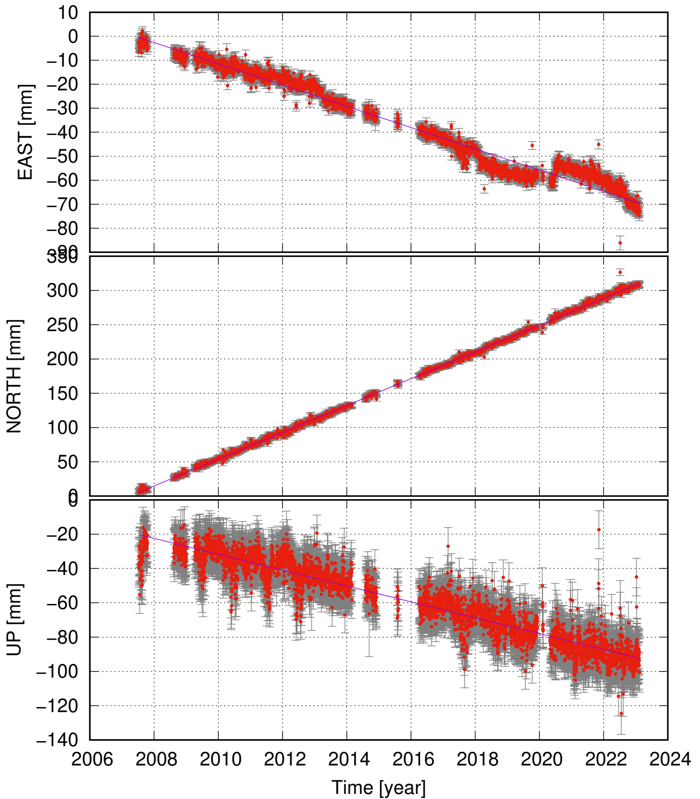
GMEY (66.54, -18.02) time series (ITRF 2014) v_e = -4.43 \pm 0.22 ; v_n = 19.55 \pm 0.13 ; v_u = -4.63 \pm 0.44 mm/yr
