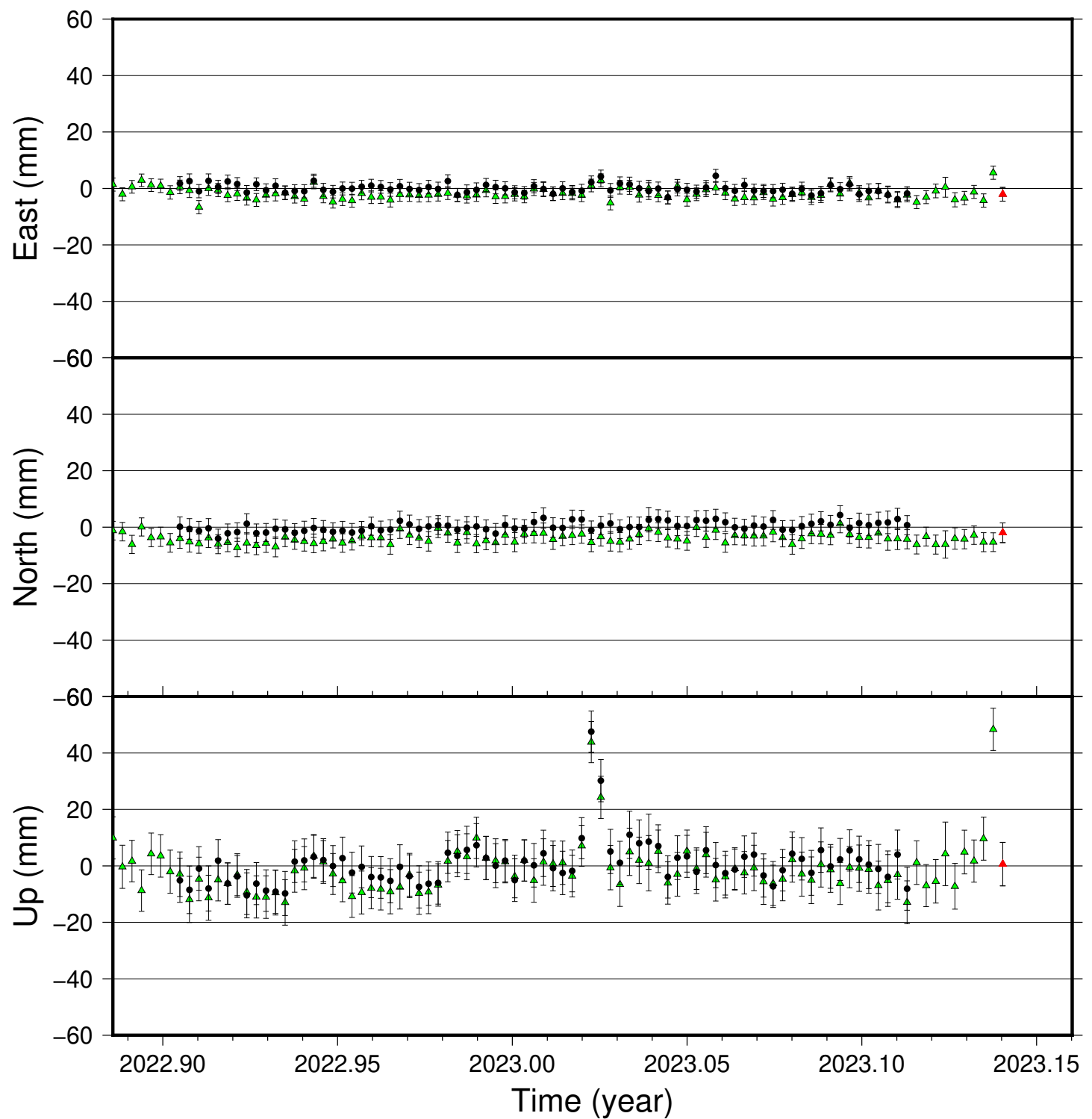
GMEY time series (IGS 2014), last 100 days
