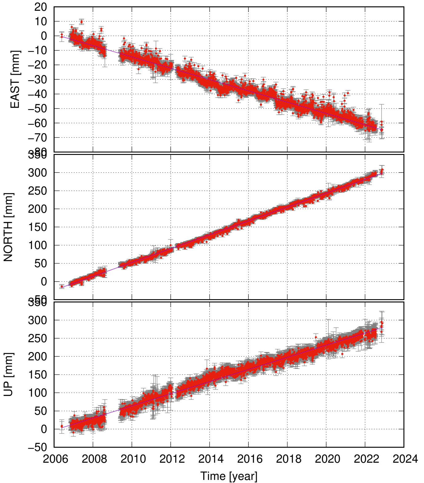
GLER (64.02, -19.80) time series (ITRF 2014) v_e = -3.89 \pm 0.15 ; v_n = 19.07 \pm 0.21 ; v_u = 16.72 \pm 0.52 mm/yr
