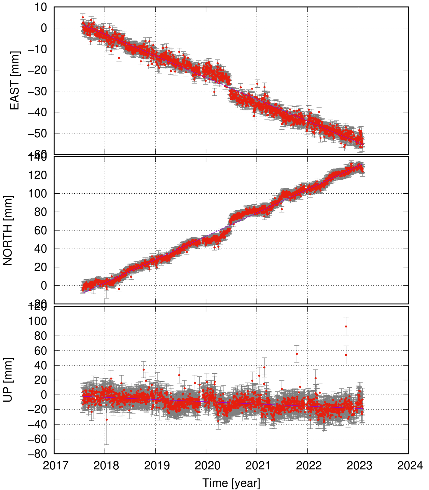
GJOG (66.17, -18.26) time series (ITRF 2014) v_e = -10.29 \pm 0.45 ; v_n = 25.36 \pm 0.72 ; v_u = -3.00 \pm 1.46 mm/yr
