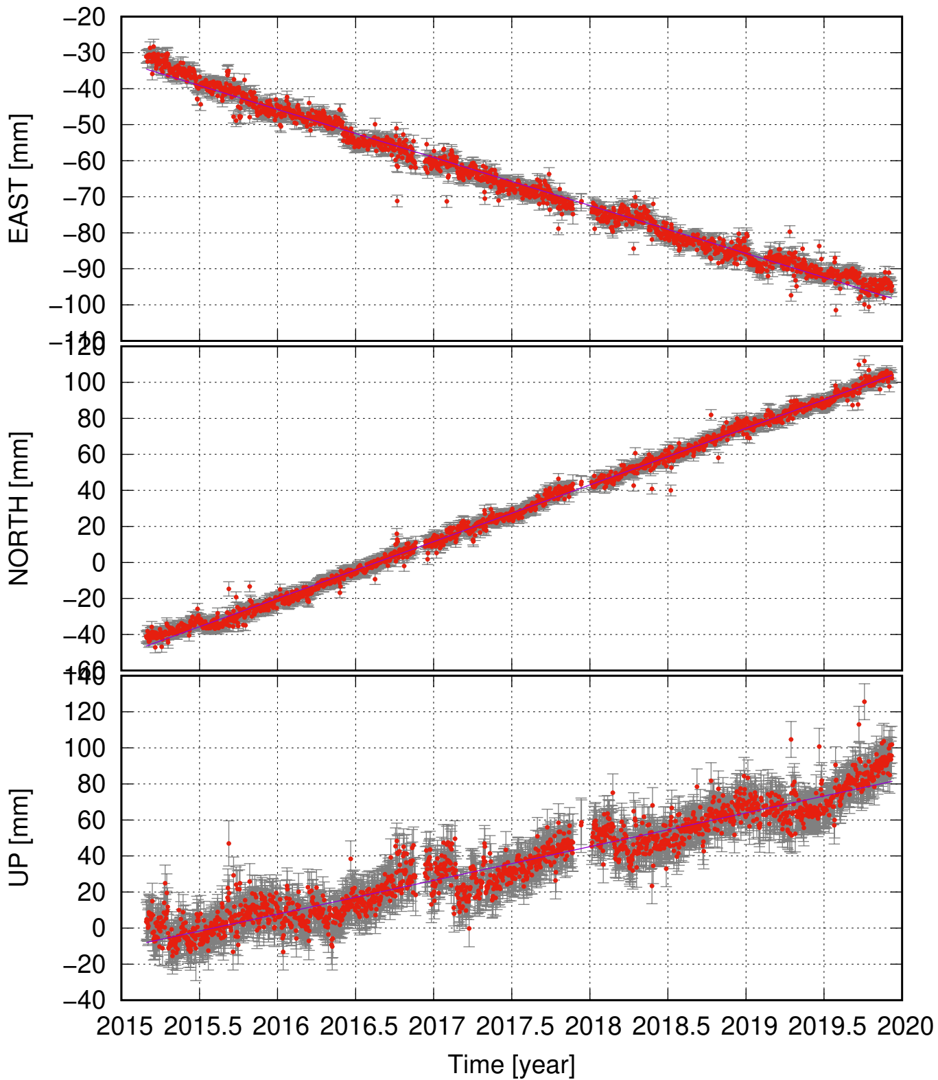
GJAC (64.83, -17.61) time series (ITRF 2014) v_e = -13.32 \pm 0.47 ; v_n = 31.49 \pm 0.56 ; v_u = 18.73 \pm 1.74 mm/yr
