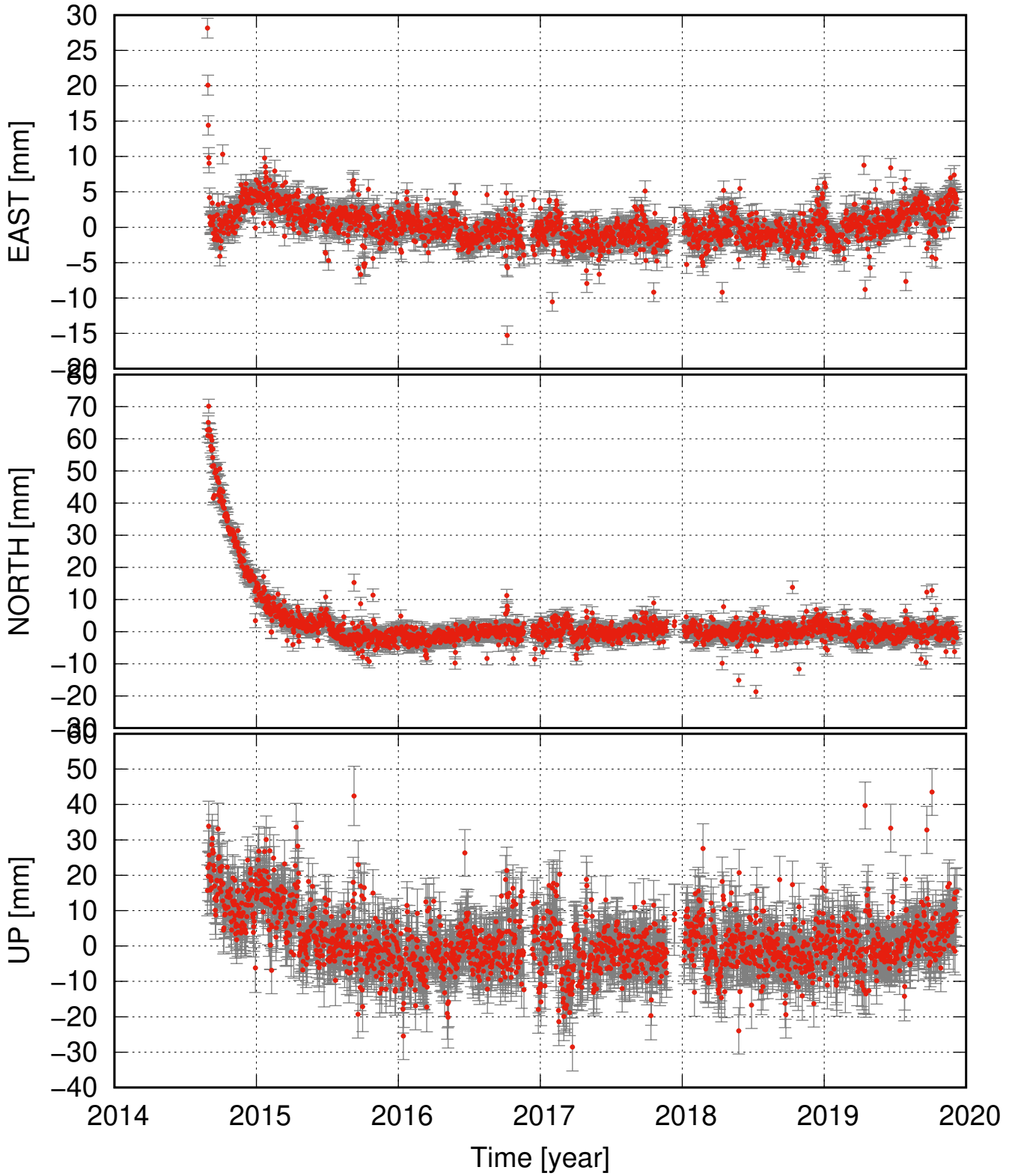
GJAC detrended and seasonal signal removed
