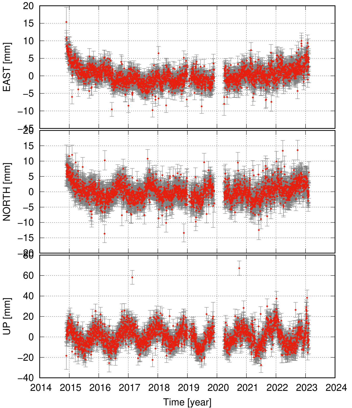
GIGO residual time series (some major events removed as well)
