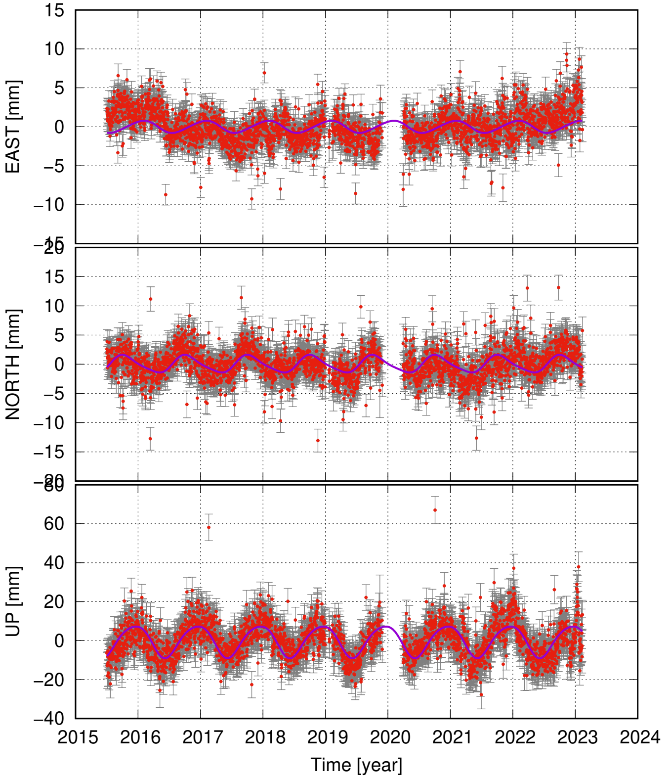
GIGO seasonal fit
