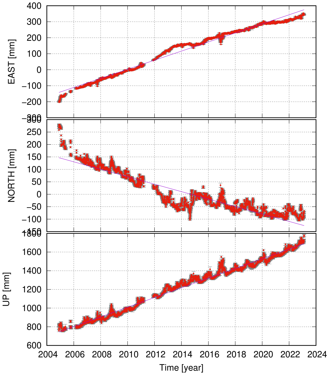
GFUM (64.41, -17.27) time series (ITRF 2014) v_e = 28.39 \pm 1.15 ; v_n = -14.97 \pm 1.77 ; v_u = 51.87 \pm 1.83 mm/yr
