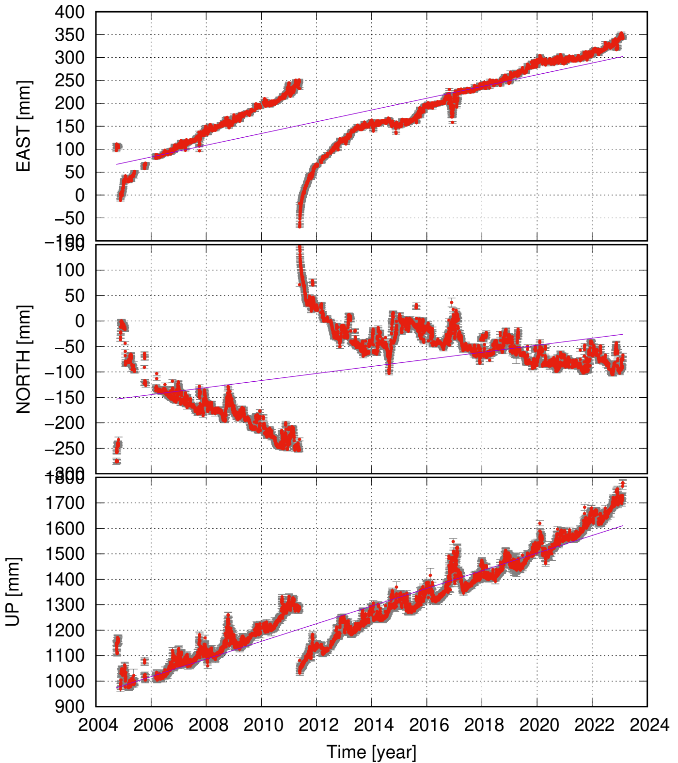
GFUM (64.41, -17.27) time series (ITRF 2014) ve = 12.82 ± 2.43; vn = 6.93 ± 3.63; vu = 34.66 ± 3.04 mm/yr
