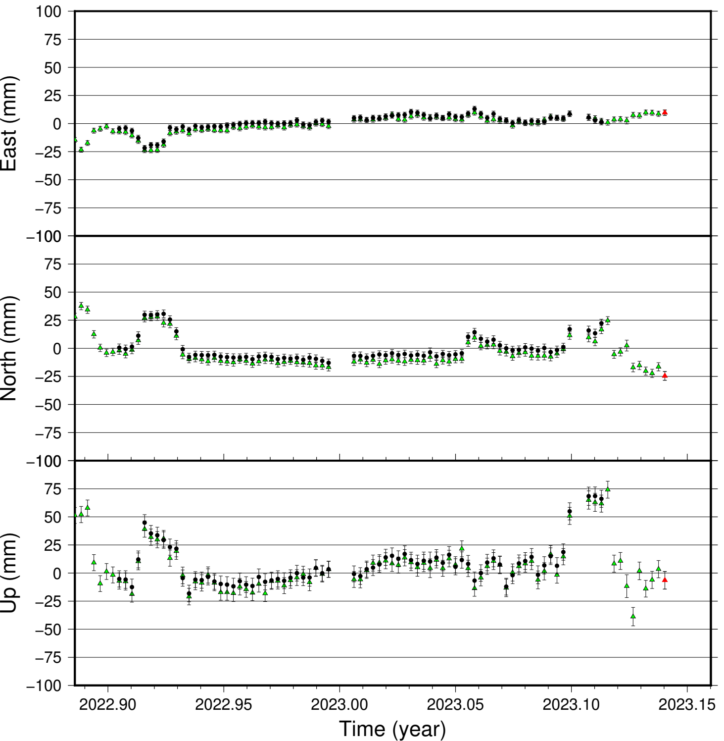
GFUM time series (IGS 2014), last 100 days
