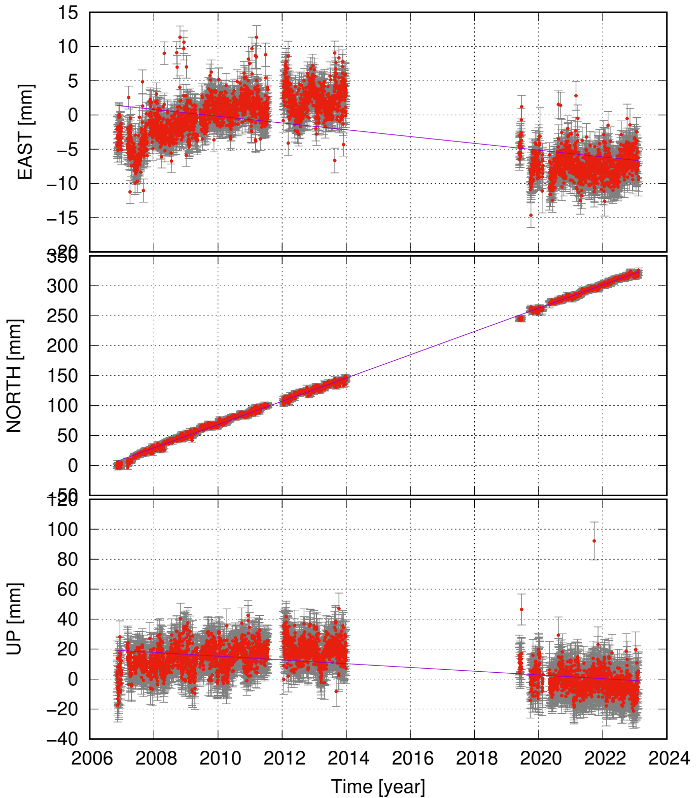
GAKE (66.08, -16.76) time series (ITRF 2014) v_e = -0.50 \pm 0.20 ; v_n = 19.43 \pm 0.19 ; v_u = -1.25 \pm 0.54 mm/yr
