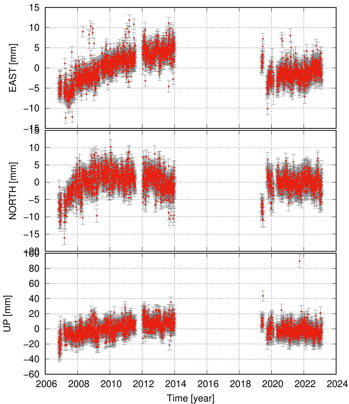
GAKE detrended and seasonal signal removed
