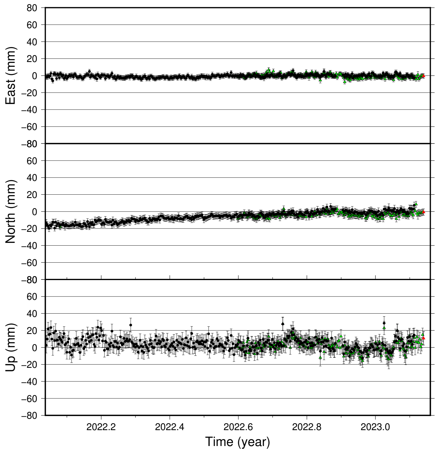
GAKE time series (IGS 2014), last 400 days
