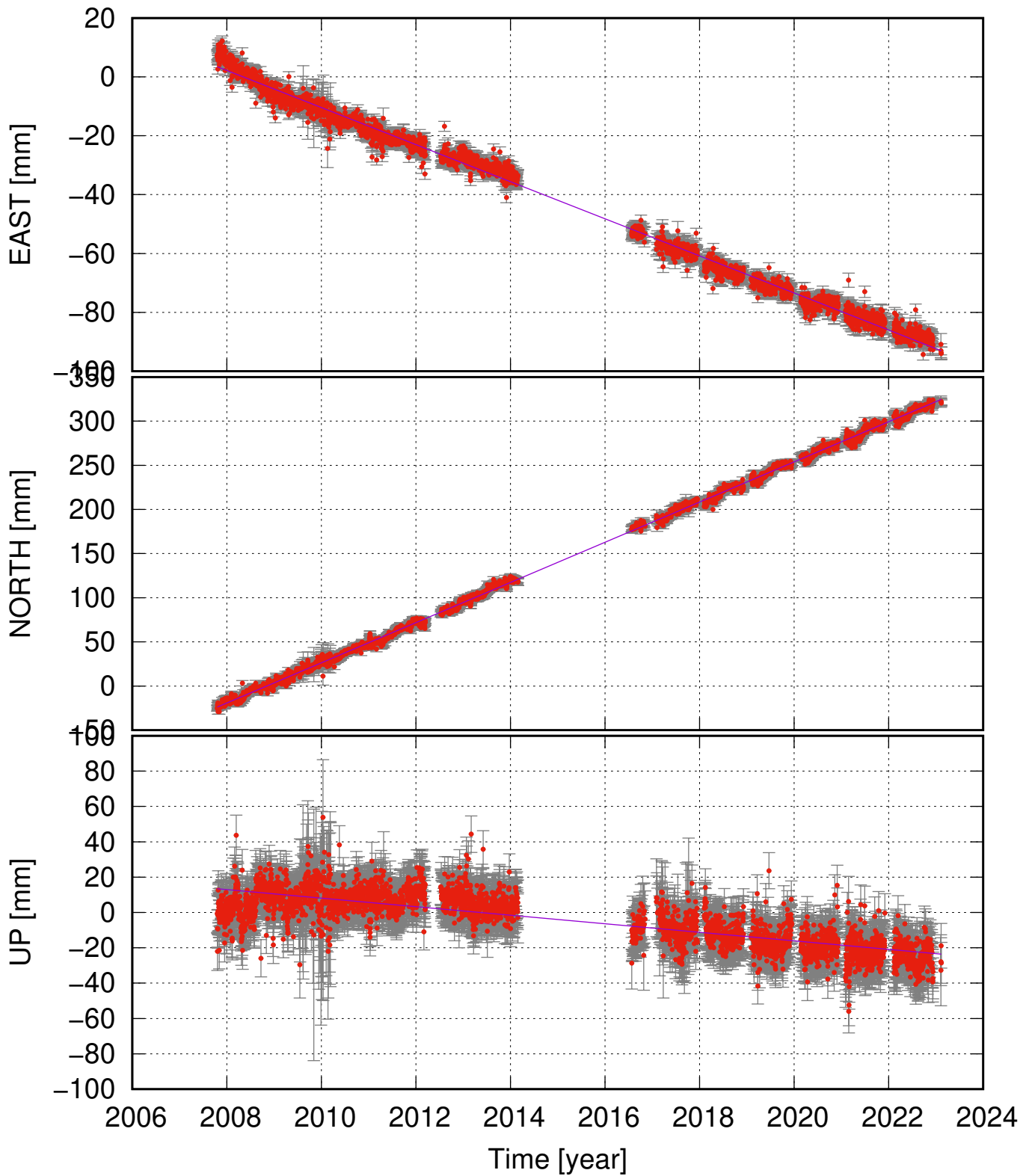
FTEY (66.16, -17.85) time series (ITRF 2014) v_e = -6.30 \pm 0.15 ; v_n = 22.76 \pm 0.20 ; v_u = -2.42 \pm 0.53 mm/yr
