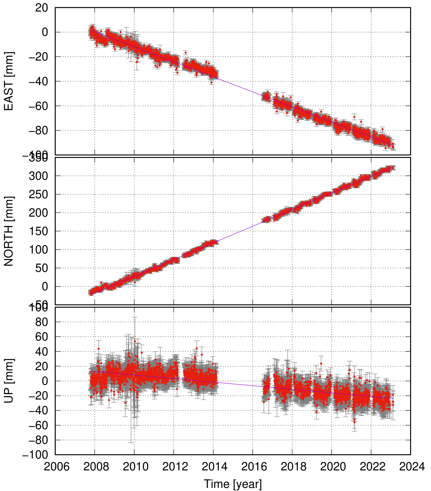
FTEY (66.16, -17.85) time series (ITRF 2014) v_e = -6.12 \pm 0.15 ; v_n = 22.59 \pm 0.23 ; v_u = -2.42 \pm 0.53 mm/yr
