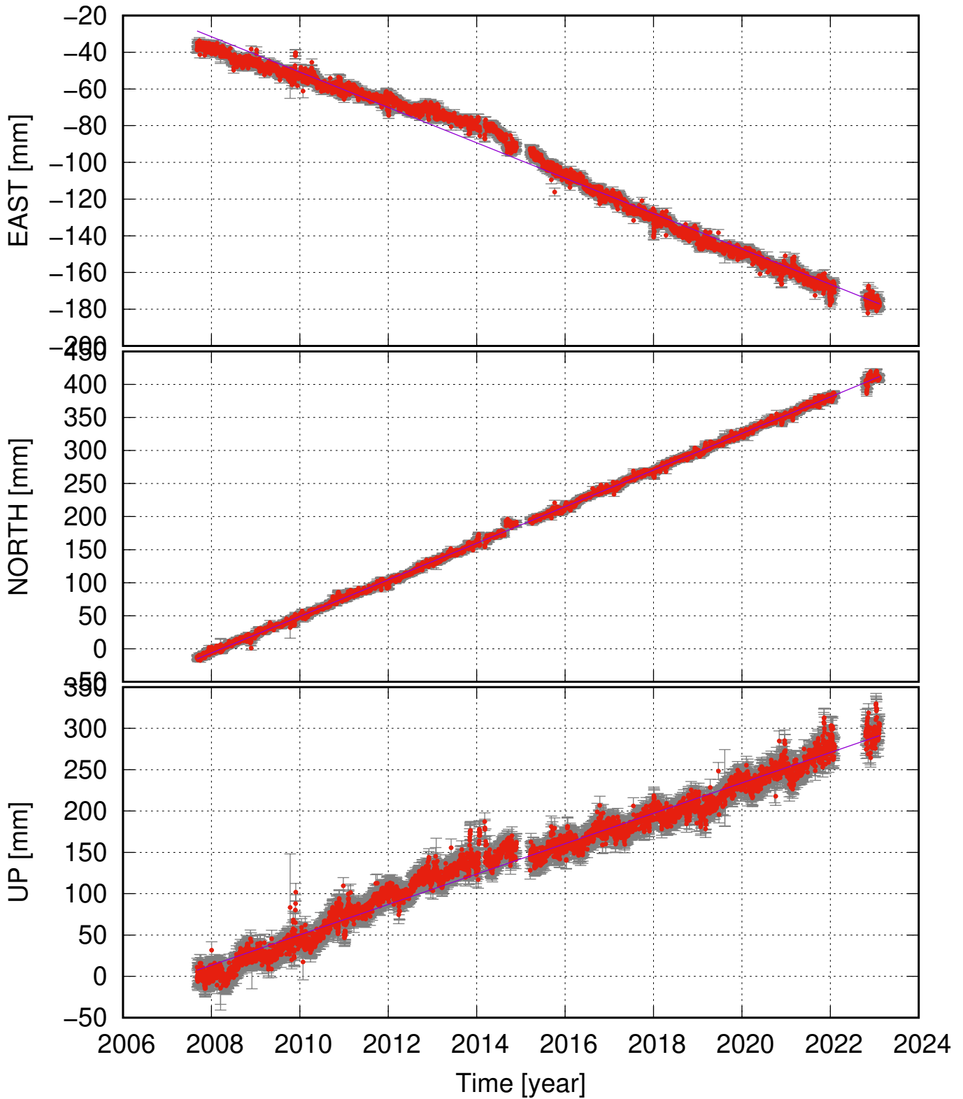
FJOC (64.87, -18.01) time series (ITRF 2014) v_e = -9.63 \pm 0.31 ; v_n = 27.66 \pm 0.19 ; v_u = 18.37 \pm 0.79 mm/yr
