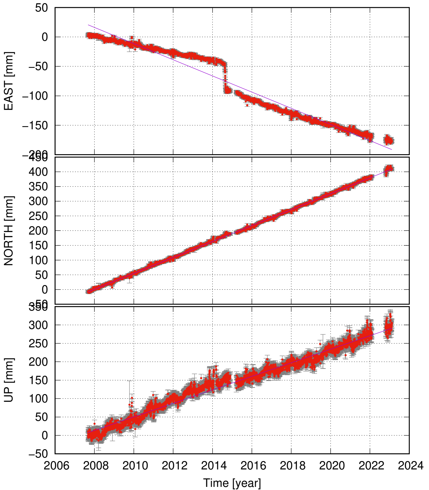
FJOC (64.87, -18.01) time series (ITRF 2014) v_e = -13.74 \pm 0.81 ; v_n = 27.05 \pm 0.20 ; v_u = 18.37 \pm 0.79 mm/yr
