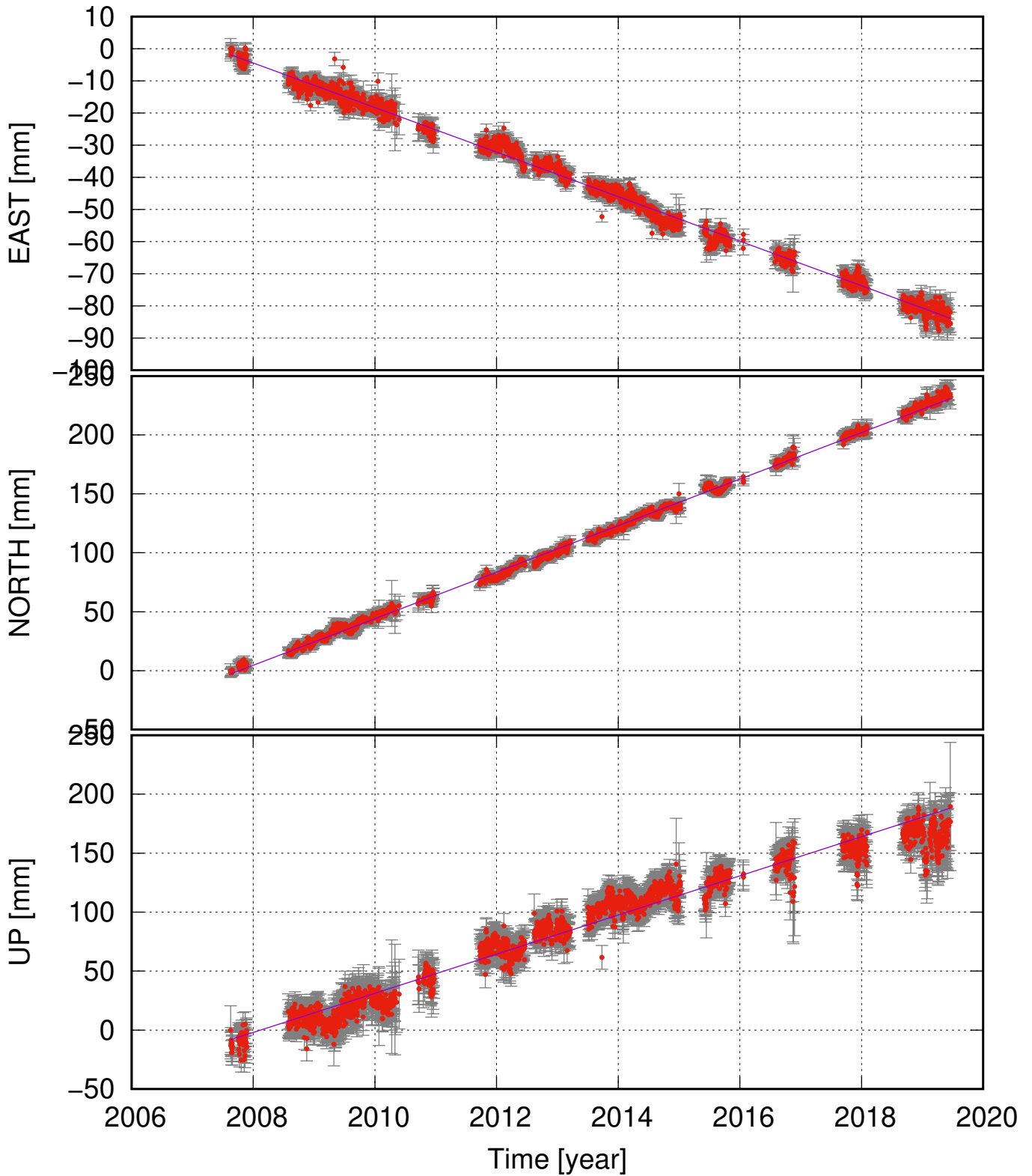
FITC (64.34, -19.59) time series (ITRF 2014) v_e = -6.93 \pm 0.16 ; v_n = 19.75 \pm 0.25 ; v_u = 16.60 \pm 0.92 mm/yr
