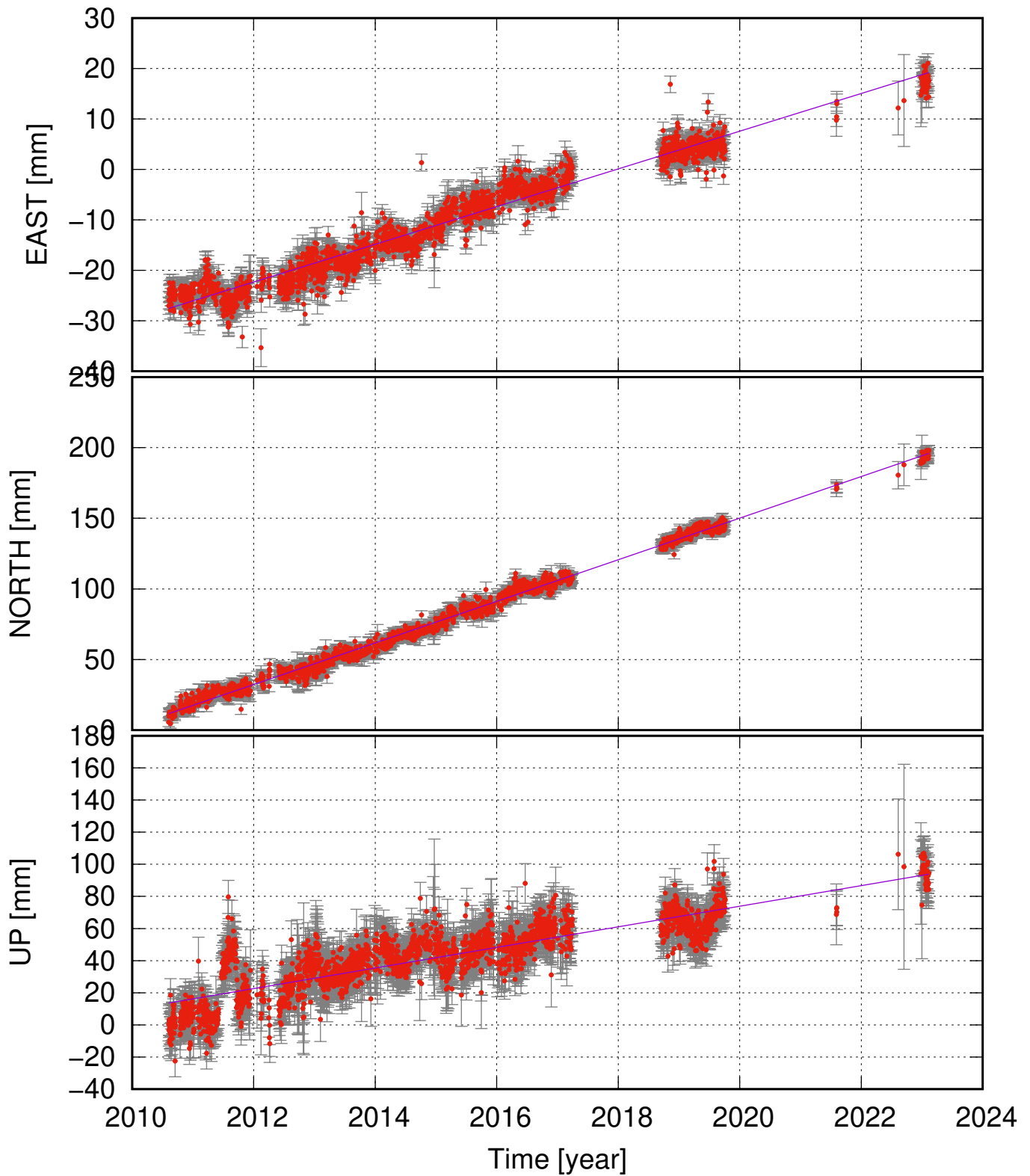
FIM2 (63.61, -19.43) time series (ITRF 2014) v_e = 3.74 \pm 0.19 ; v_n = 14.72 \pm 0.26 ; v_u = 6.40 \pm 0.86 mm/yr
