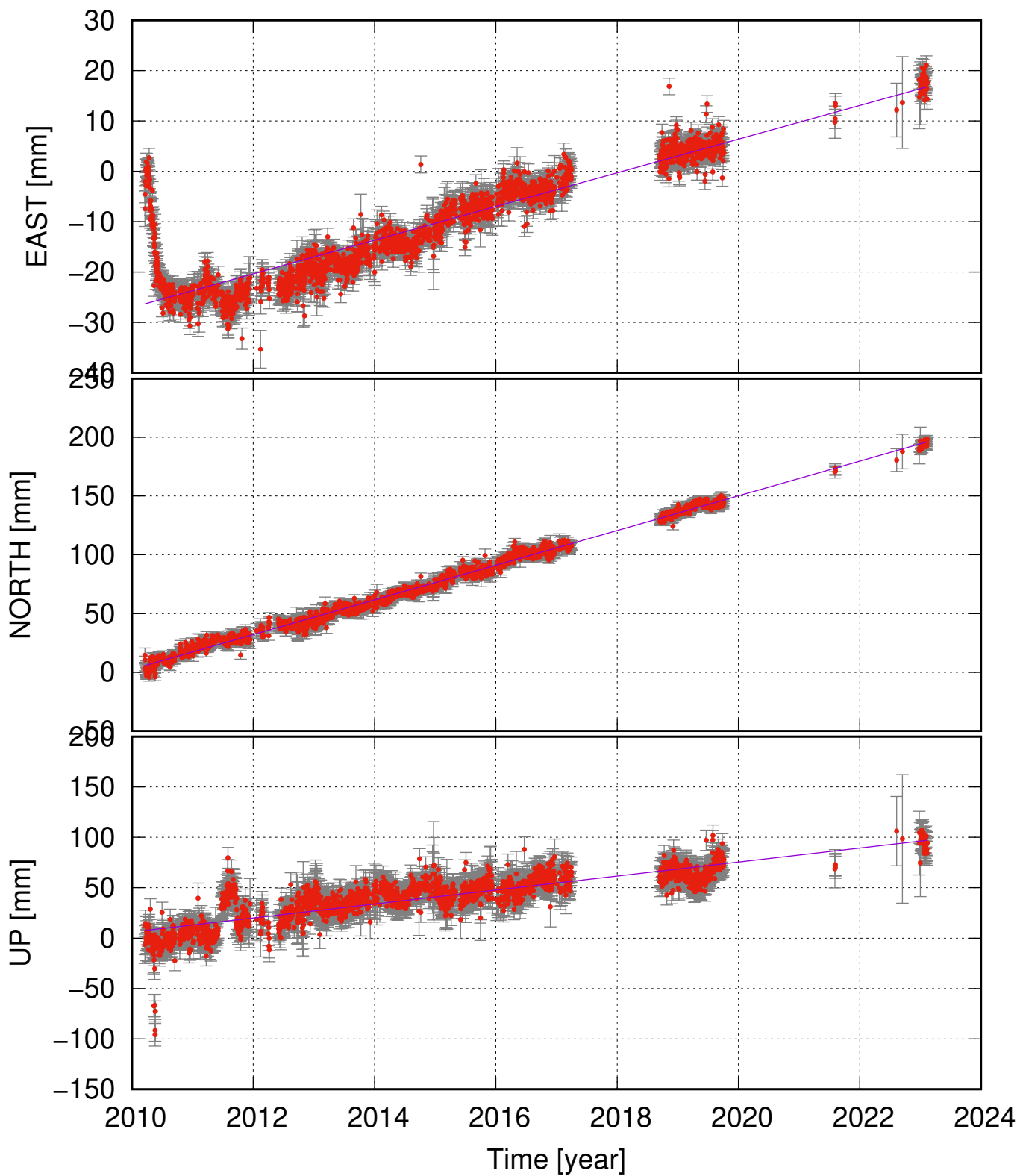
FIM2 (63.61, -19.43) time series (ITRF 2014) v_e = 3.34 \pm 0.34 ; v_n = 14.76 \pm 0.25 ; v_u = 6.94 \pm 0.92 mm/yr
