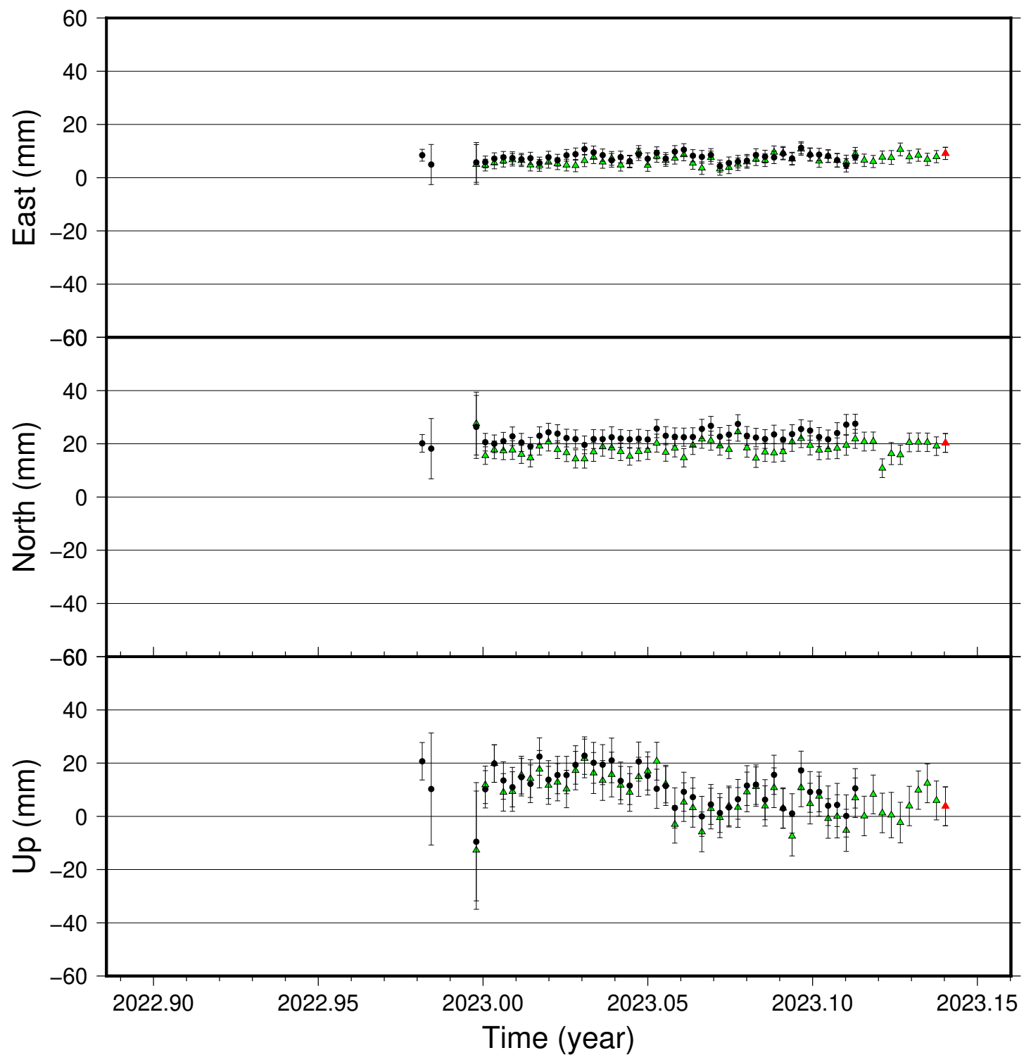
FIM2 time series (IGS 2014), last 100 days
