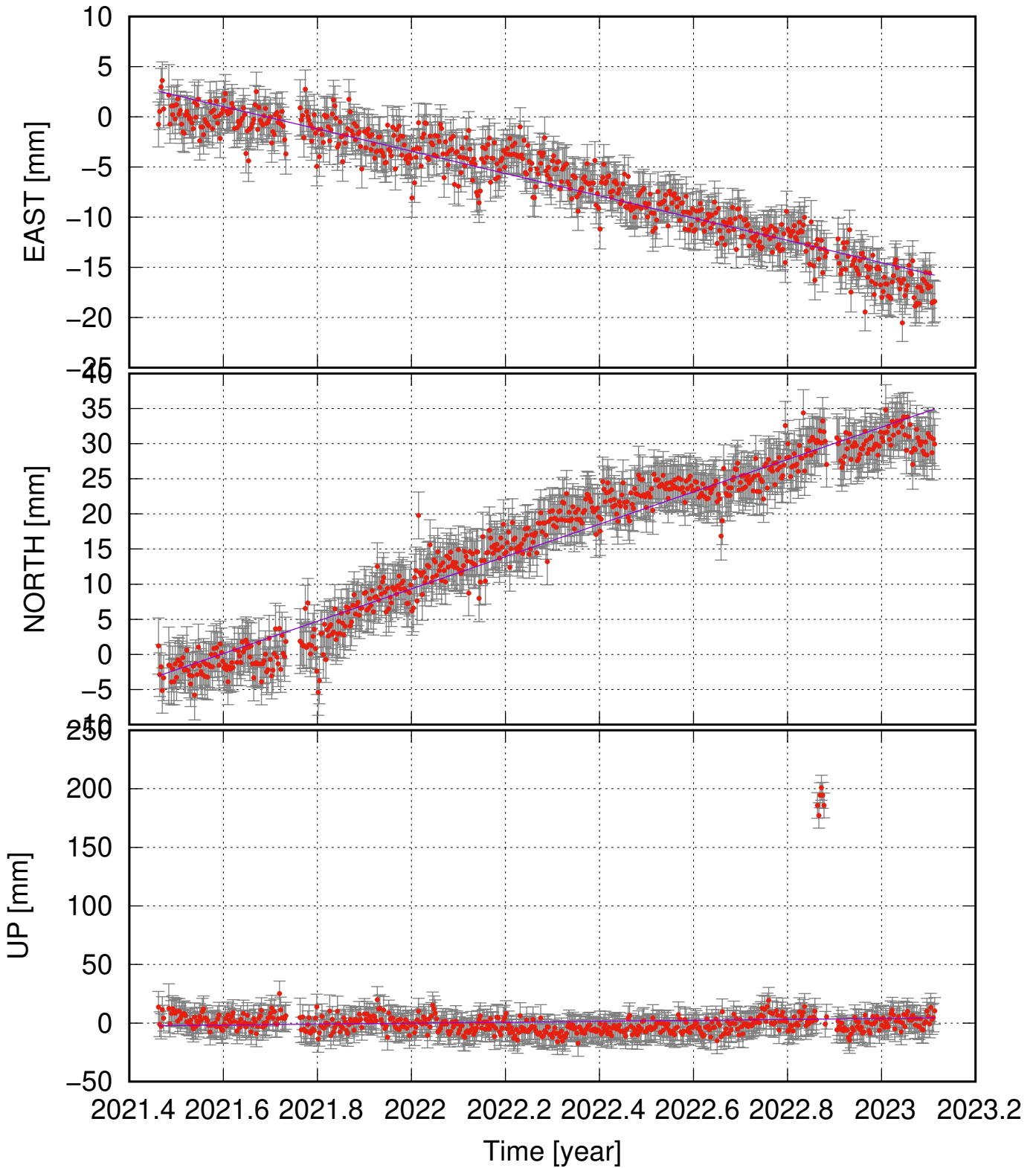
FIHO (64.69, -22.15) time series (ITRF 2014) v_e = -11.11 \pm 1.01 ; v_n = 23.01 \pm 1.52 ; v_u = 3.96 \pm 12.26 mm/yr
