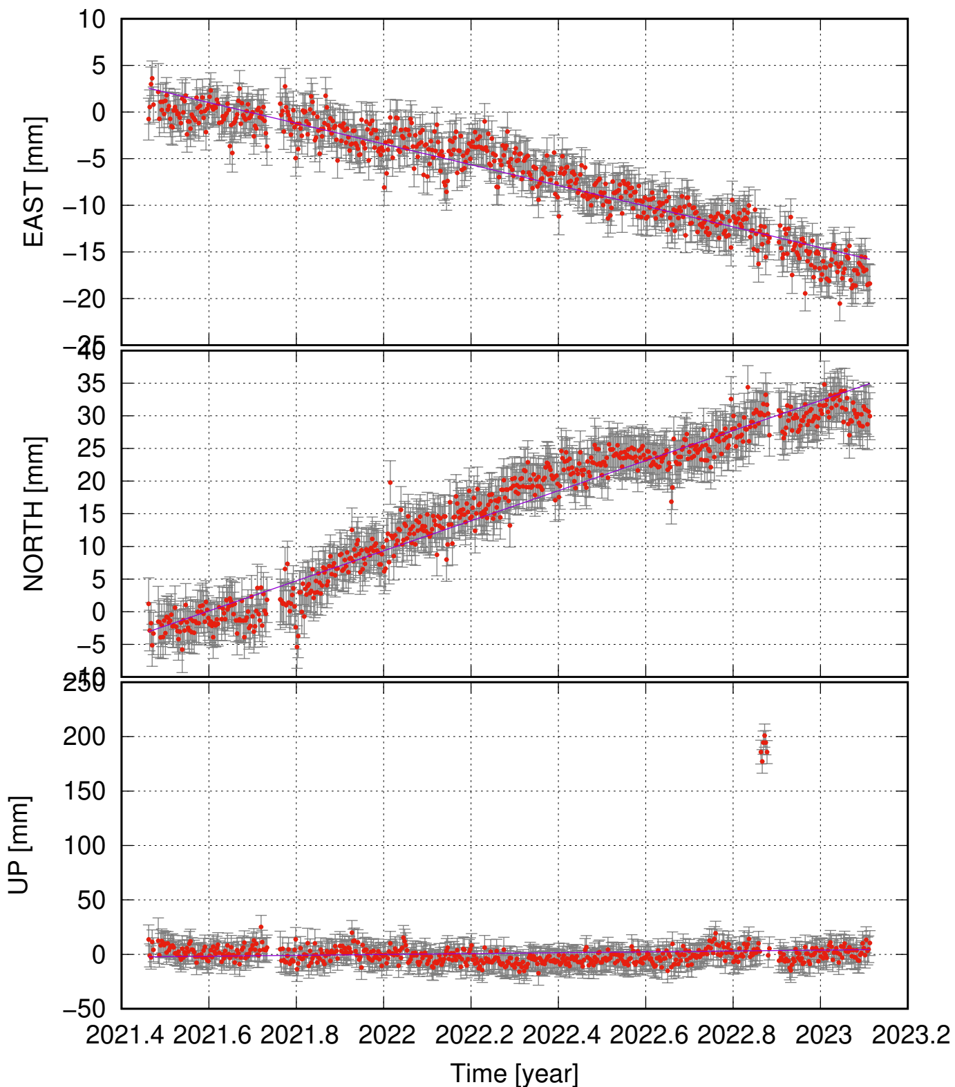
FIHO (64.69, -22.15) time series (ITRF 2014) v_e = -11.11 \pm 1.01 ; v_n = 23.01 \pm 1.52 ; v_u = 3.96 \pm 12.26 mm/yr
