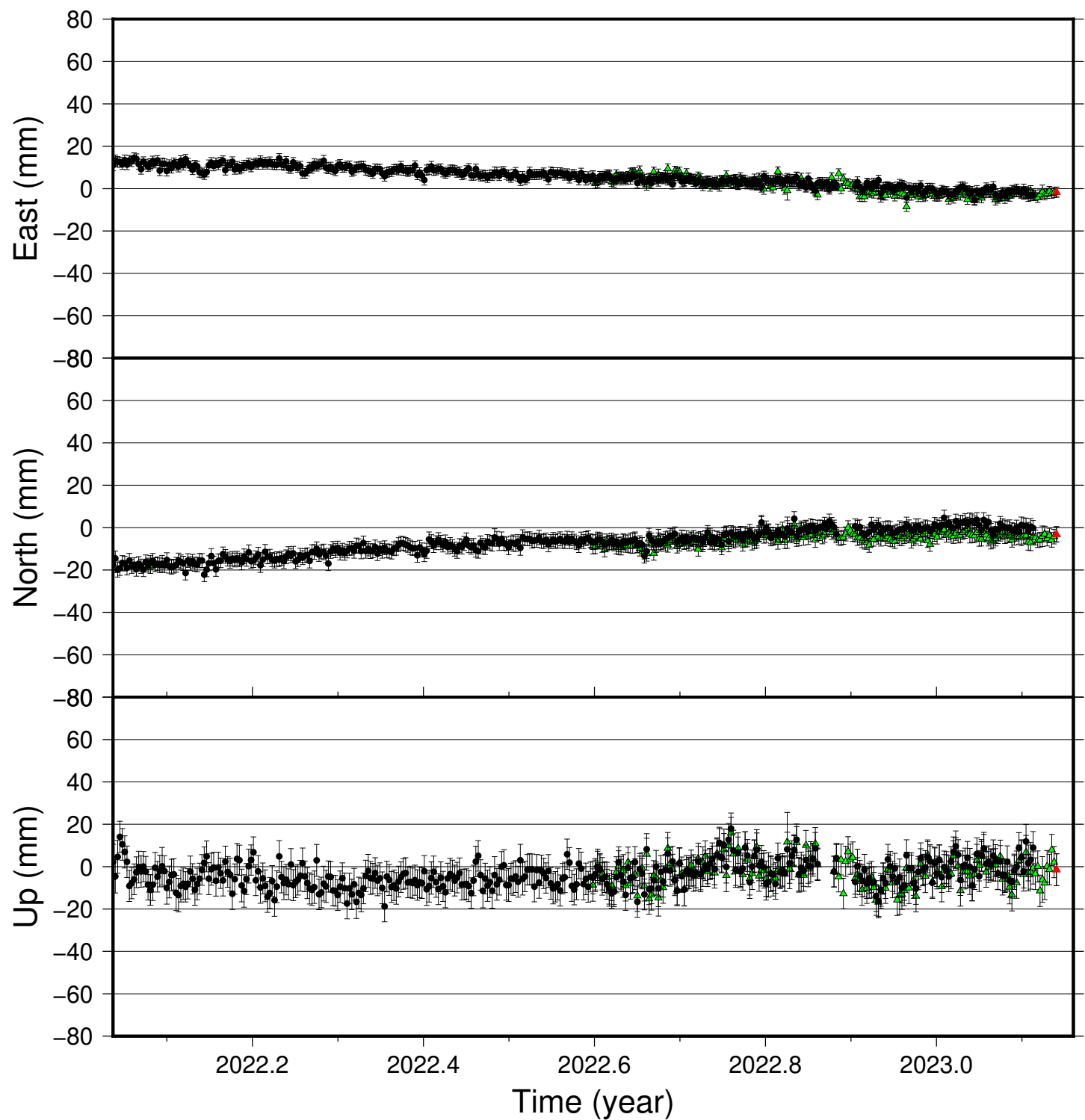
FIHO time series (IGS 2014), last 400 days
