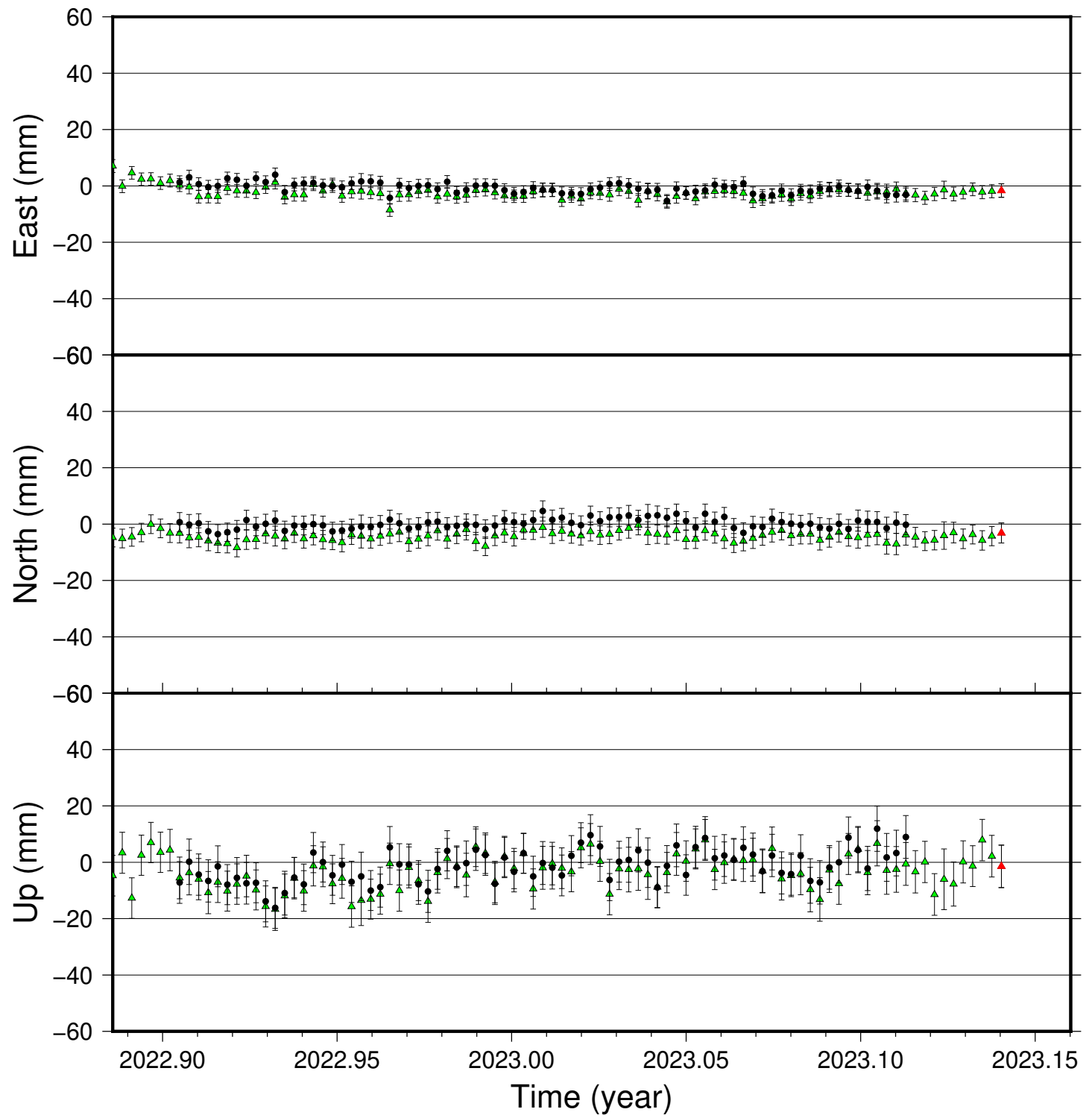
FIHO time series (IGS 2014), last 100 days
