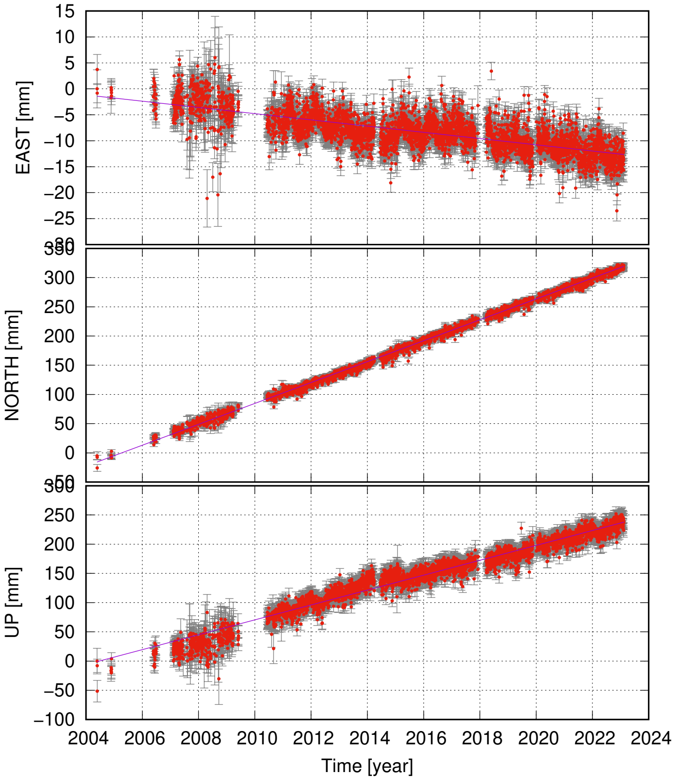
FEDG (64.03, -19.69) time series (ITRF 2014) v_e = -0.60 \pm 0.13 ; v_n = 17.89 \pm 0.21 ; v_u = 12.76 \pm 0.61 mm/yr
