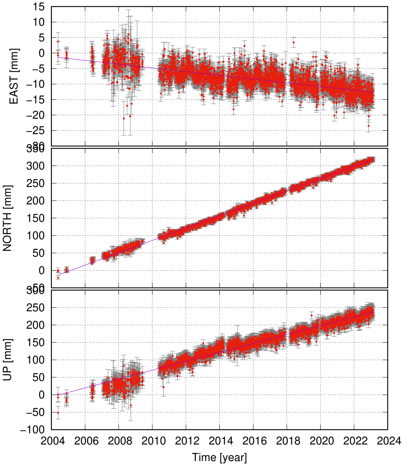
FEDG (64.03, -19.69) time series (ITRF 2014) v_e = -0.60 \pm 0.13 ; v_n = 17.71 \pm 0.24 ; v_u = 12.76 \pm 0.61 mm/yr
