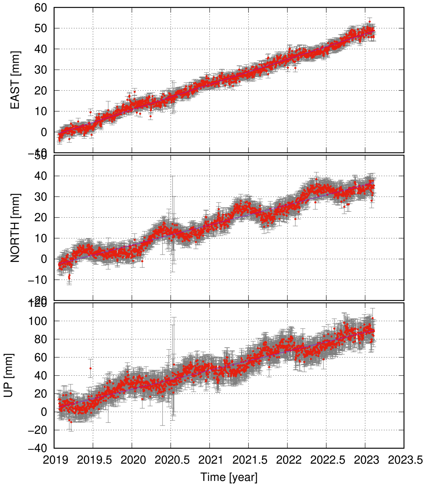
FAGC (63.87, -16.65) time series (ITRF 2014) v_e = 12.17 \pm 0.40 ; v_n = 9.66 \pm 0.69 ; v_u = 20.85 \pm 1.57 mm/yr
