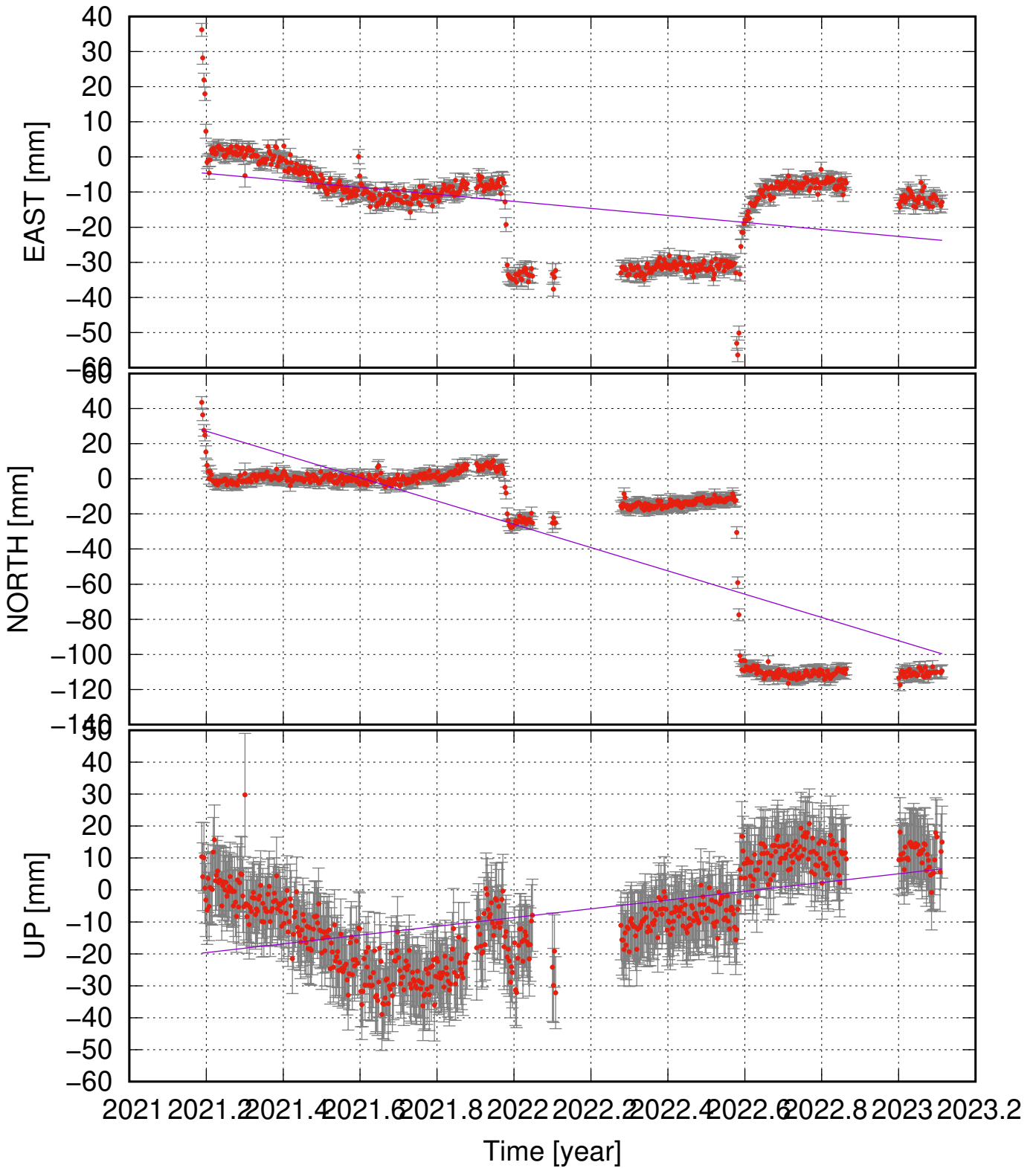
FAFC (63.91, -22.22) time series (ITRF 2014) v_e = -9.97 \pm 5.65 ; v_n = -66.28 \pm 14.02 ; v_u = 13.73 \pm 6.14 mm/yr
