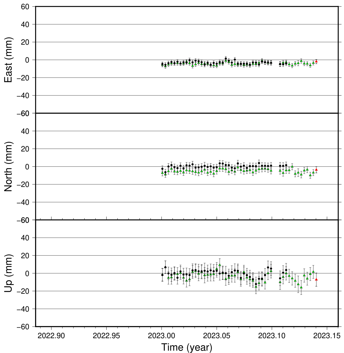
FAFC time series (IGS 2014), last 100 days
