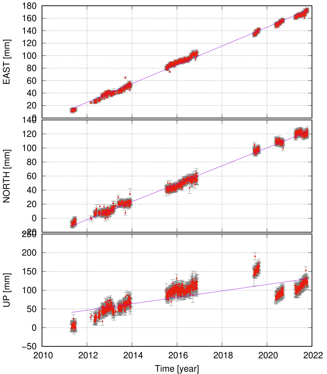
EYVI (64.23, -15.80) time series (ITRF 2014) ve = 15.06 ± 0.30; vn = 12.78 ± 0.32; vu = 8.57 ± 2.11 mm/yr
